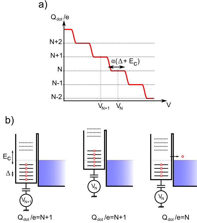
Figure 4: a) Coulomb blockade: the charge of a quantum dot presents quantized steps as a function of the gate voltage controlling the potential in the dot. b) single-charge emission with a quasi-metallic quantum dot: the dot is rapidly brought out of equilibrium by changing the gate voltage from V_{N+1} to V_N . An electron from one of the levels promoted above the Fermi energy can tunnel out of the dot: a single charge is emitted.
