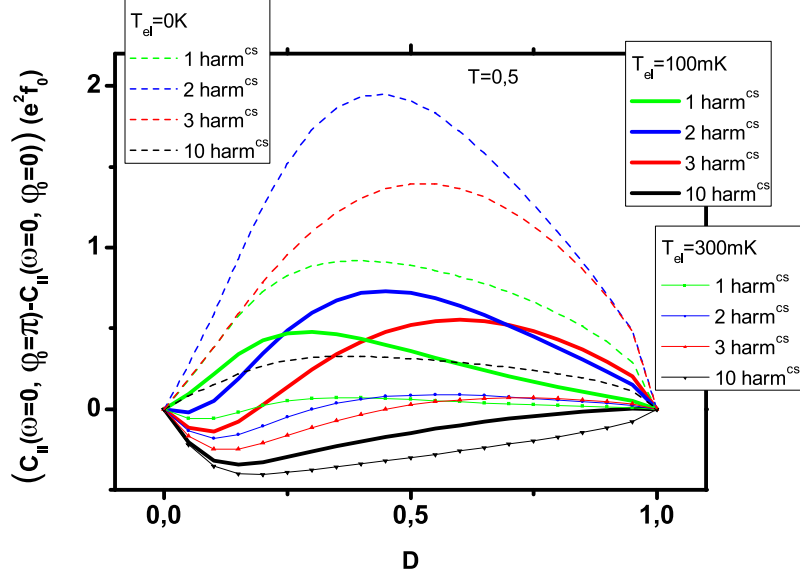
Figure 3.9: Effect of the temperature on the difference C_{II}(\omega=0, \phi_0=\pi) - C_{II}(\omega=0, \phi_0=0) (plotted as a function of the transmission D ; T=0.5 ). Dashed lines: zero temperature limit T_{el} = 0 K. Full lines: T_{el} = 100 mK. Thin lines with symbols: T_{el} = 300 mK. The colors correspond to the number of harmonics in the excitation drive: 1 (green), 2 (blue), 3 (red) and 10 (black). For any shape of the drive, the measured difference diminishes with the temperature.
