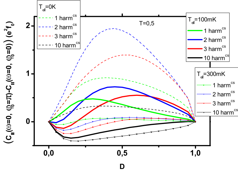
Figure 3.9: Effect of the temperature on the difference C_{I_1 I_1}(\omega = 0, \phi_0 = \pi) - C_{I_1 I_1}(\omega = 0, \phi_0 = 0) (plotted as a function of the transmission D ; T = 0.5 ). Dashed lines: zero temperature limit T_{el} = 0 K. Full lines: T_{el} = 100 mK. Thin lines with symbols: T_{el} = 300 mK. The colors correspond to the number of harmonics in the excitation drive: 1 (green), 2 (blue), 3 (red) and 10 (black). For any shape of the drive, the measured difference diminishes with the temperature.
