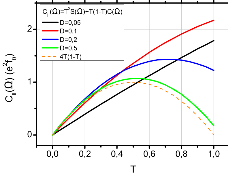
Figure 3.7: Variation of C_{I_1 I_1}(\omega = \Omega) with the central QPC transmission T , for several values of D . For large D , the noise becomes comparable to the T(1 - T) limit (dashed line).
