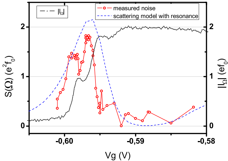
Figure 3.19: Noise of the single electron source versus V_g for sample S434-8 . Red circles: experimental data; blue dashed line: scattering model, using the QPC transmission law with a resonance at V_g = -0.586 V depicted in Fig.3.17. Black line with symbols: modulus of the first harmonic of the average AC current, for 2eV_{exc} = \Delta .
