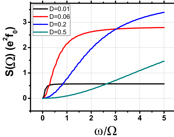
Figure 2.3: Calculated noise as a function of the measurement frequency in the injection regime: 2eV_{exc} = \Delta , \phi_0 = 0 . We have taken f_0 = 1.5\text{ GHz} (that is \hbar\Omega/k_B = 0.07\text{ K} ), and \Delta = 4\text{ K} .
