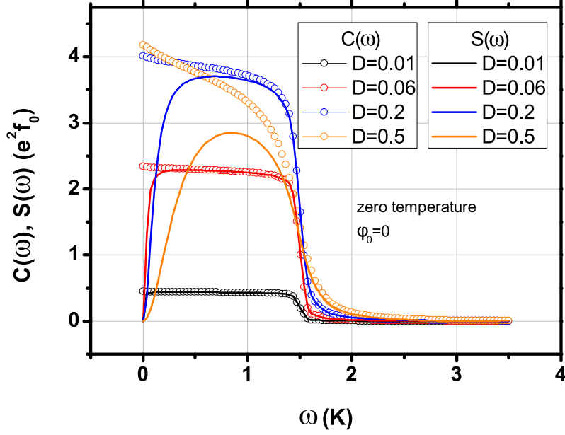
Figure 3.5: Variation of C(\omega) (circles) and S(\omega) (full lines) with the measurement frequency, in the \phi_0 = 0 case, at zero temperature. For small transmissions D , C(\omega) and S(\omega) coincide at finite frequency. Here, \Delta = 3 K, and \Omega = 70 mK.
