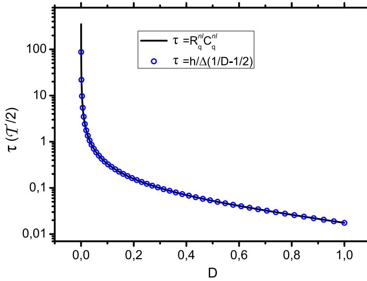
Figure 1.10: Calculated escape time as a function of the QPC transmission. The black line corresponds to the escape time given by the formula \tau = R_q^{nl} C_q^{nl} . The blue circles correspond to Eq.1.49. For low transmissions, the escape time becomes larger than the half-period \mathcal{T}/2 .
