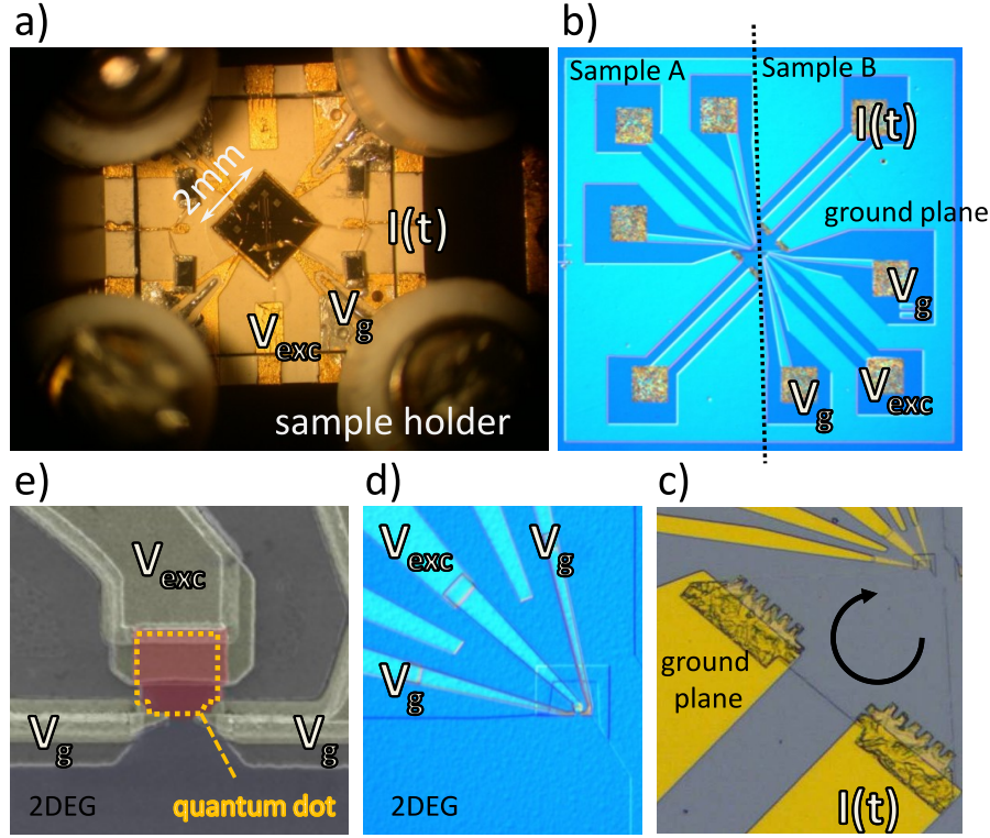
Figure 2.12: Pictures of sample S528-11 : a) optical view of the sample installed in the sample holder. b) , c) , d) optical views with increasing zoom of the chip. As seen on b) , each chip contains two samples. The black arrow in c) depicts to the chirality of electronic transport when an strong perpendicular magnetic field is applied. e) SEM view of the mesoscopic capacitor (with false colors). The quantum dot is highlighted in red.
