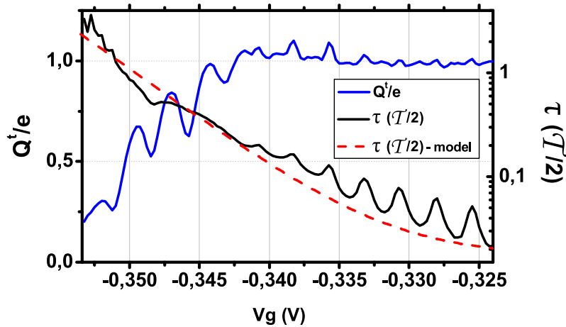
Figure 1.19: Escape time and average transfered charge as a function of V_g , for 2eV_{exc} = \Delta . The red dashed line corresponds to simulations using the ideal non-linear QPC transmission law. Discrepancies appear at smaller negative voltages, where the ideal transmission law does not exactly reproduce the experimental data.
