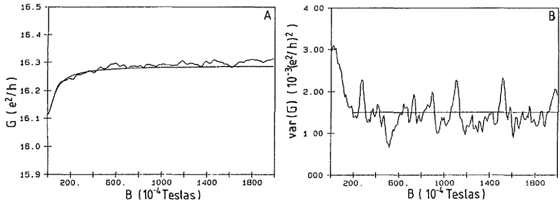
Figure 3.8: A: mean conductance obtained from figure 3.7 and the weak localization fit [72]. B: the variance over the 46 disorder configurations (at fixed magnetic field) as a function of the magnetic field. Extracted from [90].
