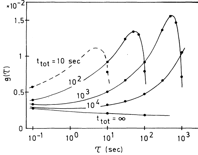
Figure 1.11: Evolution of the relaxation time spectrum ( g(\tau) vs \tau ) for different total time t_{\text{tot}} = t + t_w the system is kept at fixed temperature ( T = 23\text{K} ) for a Cu:Mn spin glass (4 at % Mn). The relaxation time spectrum is normalized according to \int g(\tau) d \log \tau = 1 . Extracted from [21].
