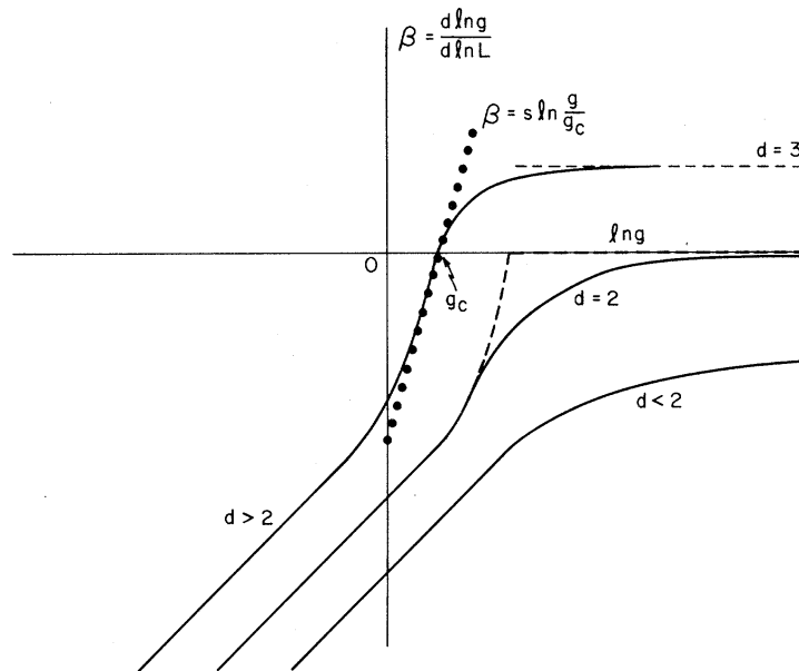
Figure 5.1: Plot of the scaling function as a function of \log g for one, two and three dimensional systems. The absence of fixed points for a finite value of conductance in one and two dimensions leads to the absence of metallic regime in the asymptotic limit. Extracted from [120].
