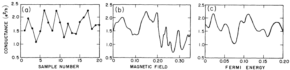
Figure 3.9: Illustration of the ergodic hypothesis that states that the statistical ensembles of the conductance with respect to disorder or magnetic field (or the Fermi energy) are similar. Numerical data extracted from [89].
