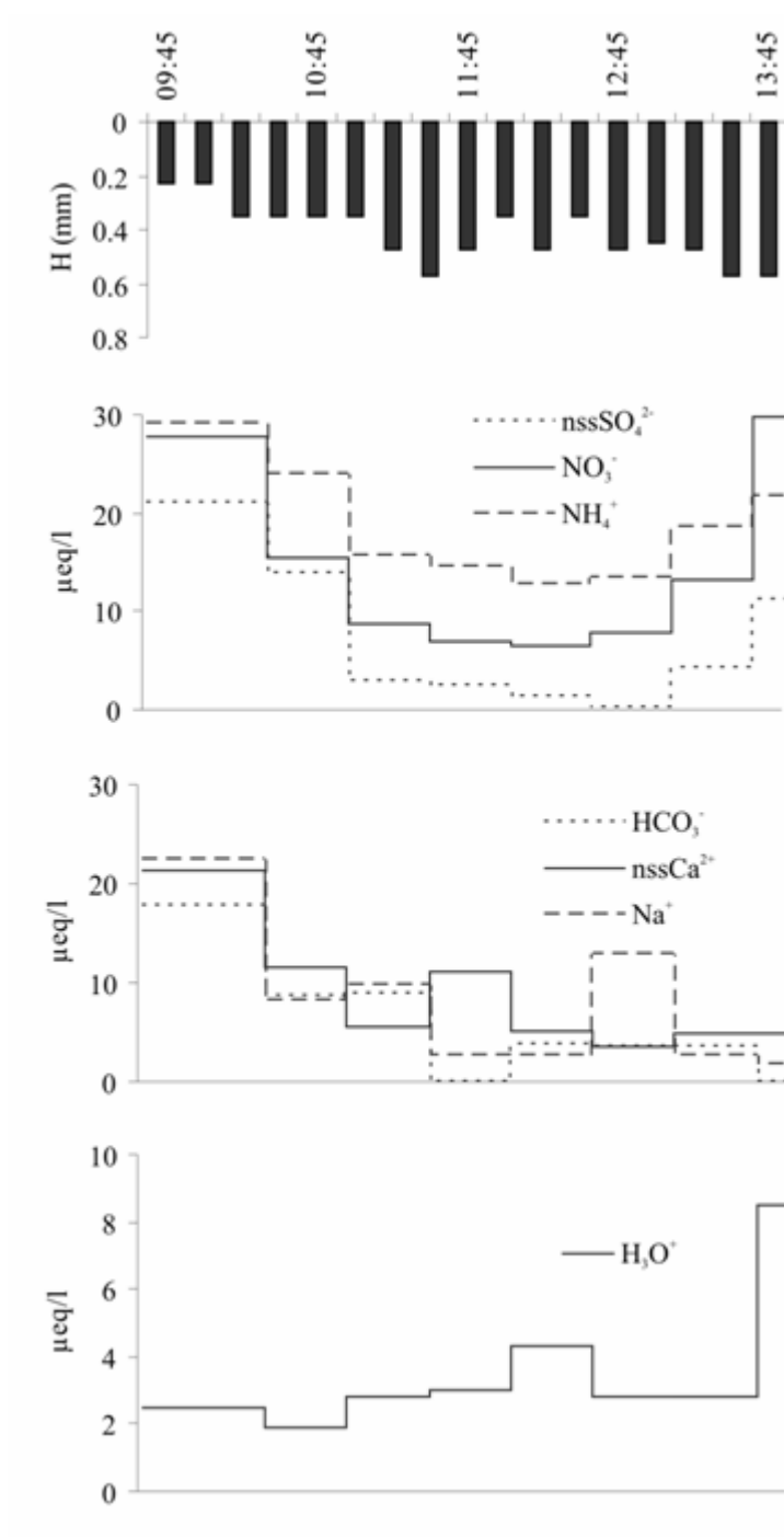
Figure II-13: Evolution of the chemical content and rainfall height for the 11/04/2006 event coming from sector 2.
