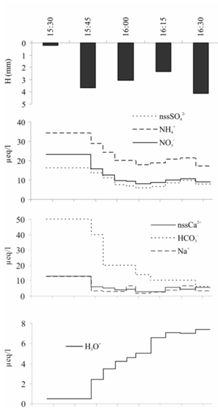
Figure II-15: Evolution of the chemical content and rainfall height for the 07/05/2006 event coming from sector 4.
