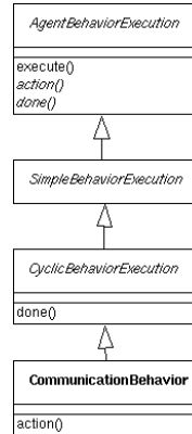
FIGURE 2.16 – Comportement de communication.
