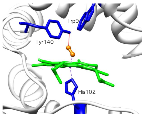
Figure 3.4: Close-up view of the heme prosthetic group (green) of Tt -SONO, histidine, tyrosine, tryptophan residues coordinating its iron with O_2 ligand (orange). Red line depicts that the phenolic OH of Tyr140 is within hydrogen bonding distance of the oxy ligand. His102 (proximal ligand of the heme Fe^{2+} ), Tyr140, and Trp9 are shown in blue. PDB ID is 1XBN and the figure was generated using Chimera.
