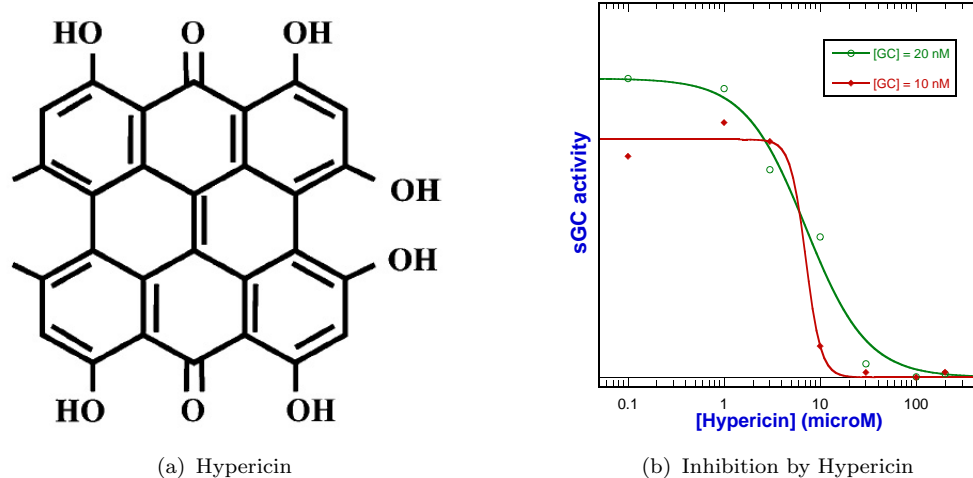
Figure 2.29: (a) Chemical structure of Hypericin and (b) Inhibition of the activity of sGC from beef lung by hypericin. K_i = 7 \mu\text{M} .
