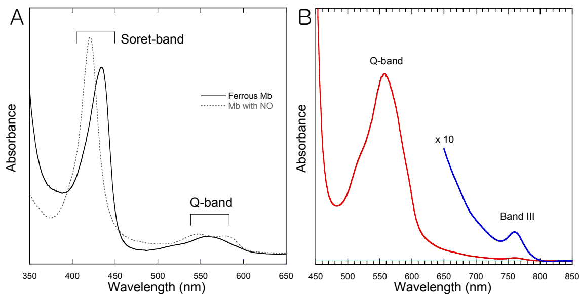
Figure 1.5: A) Absorption spectra of the Mb in the reduced (solid line) and NO-bound form (dotted line), B) Absorption spectra of the reduced Mb in near-IR region.
