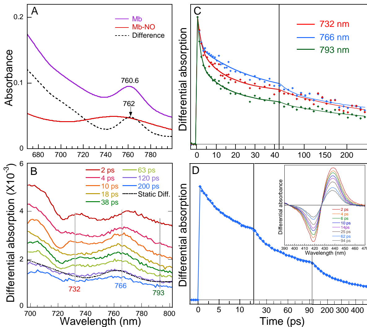
Figure 7.1: A) Equilibrium absorption spectra of Mb in the absence and presence of NO at the near IR region. [Mb] = 4 mM, NO 10 % in gas phase. B) Raw transient spectra at selected time delays, these spectra are not offset. Static absorbance difference spectrum (dotted) is included. C) Normalized kinetics at selected wavelengths, indicated by the dotted lines in panel B. D) Kinetics of NO rebinding probed by Soret absorption. SVD analysis of the entire time-wavelength matrix data and raw transient spectra (inserts) at given time delays for Mb in water.
