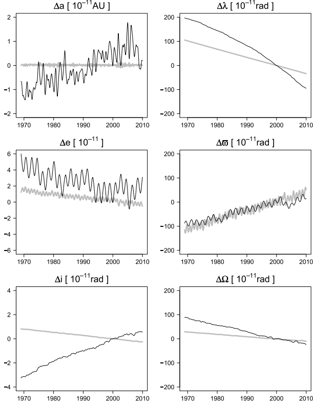
Fig. 5. Perturbation induced on the orbital elements of Earth (in gray) and Mars by the test model after removing from the test model the 300 most important perturbors.
