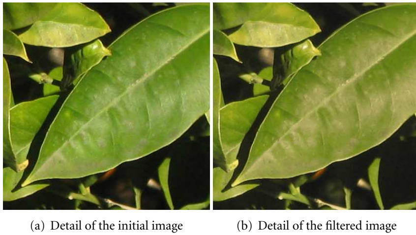
Figure 8.11: Color change.
