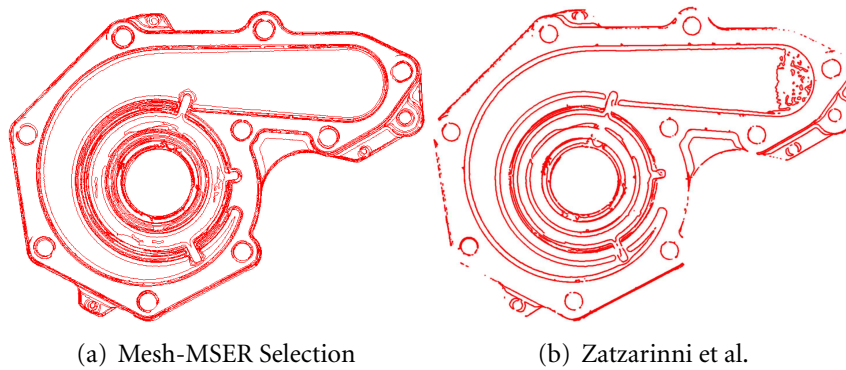
Figure 6.10: Result of Mesh-MSER on the pump mesh and comparison with the method by Zatarinni et al. ([KST09]).
