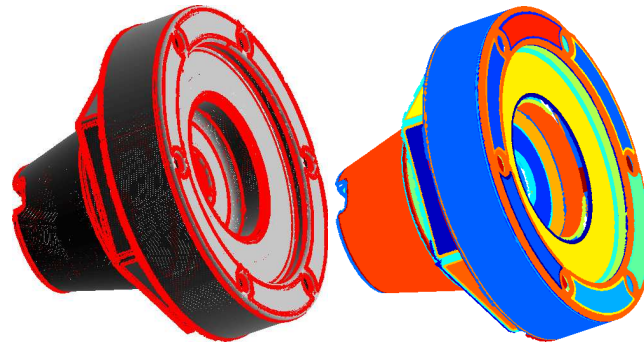
Figure 1.3: Line extraction (left) and segmentation (right) obtained by Mesh-MSER
