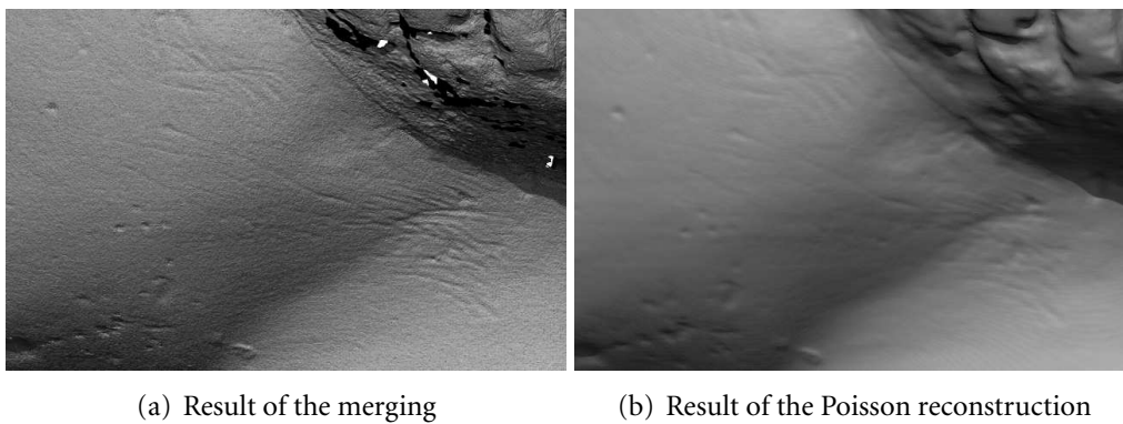
Figure 4.14: Comparison of the mesh obtained by merging and by Poisson reconstruction on a detail of nefertiti's cheek. In this case, Poisson Reconstruction suppresses registration artefacts but smooths out the details.
