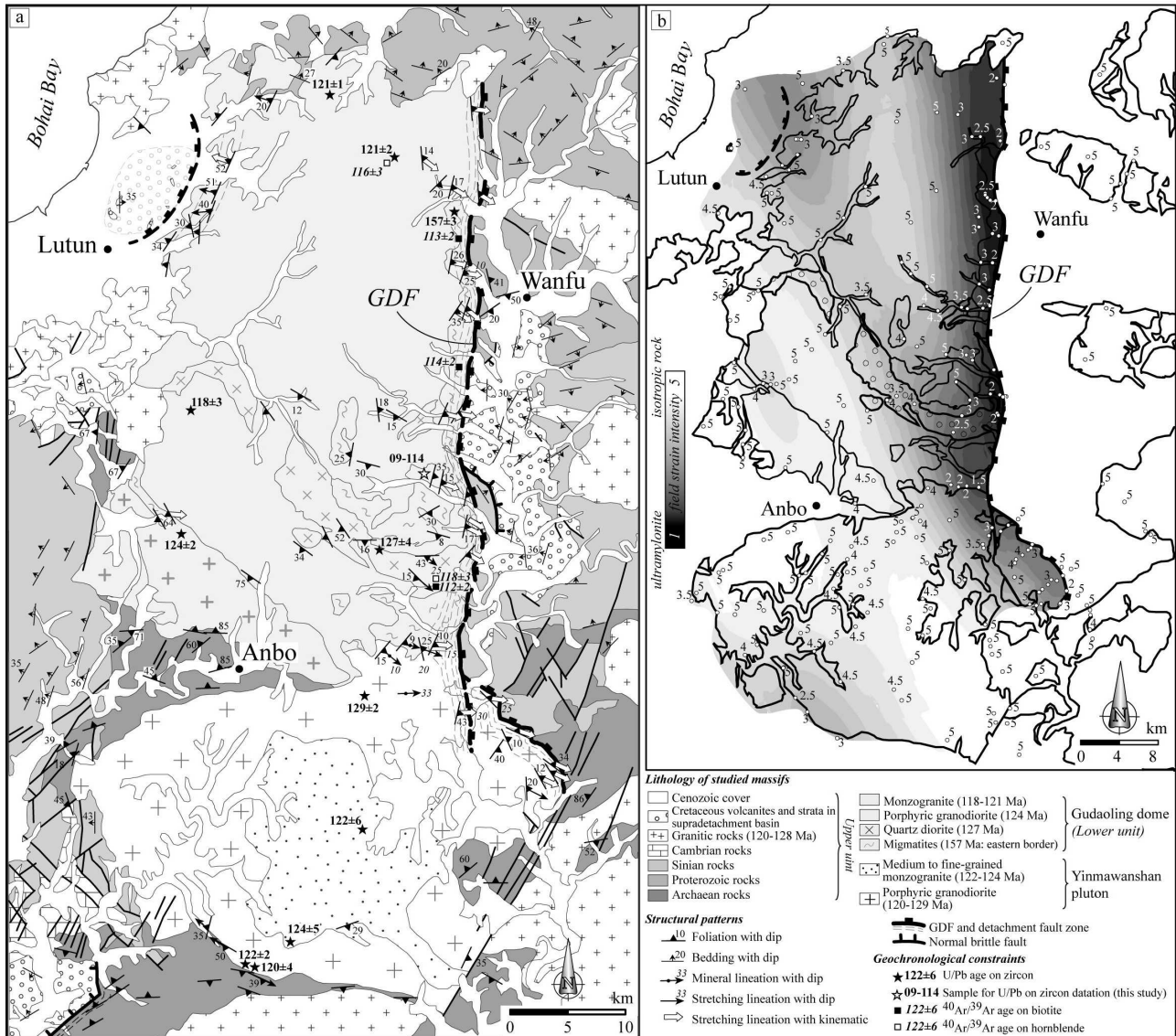
Figure 4.11: (a) Structural map of the Gudaoling and Yimwanshan massifs. U/Pb ages on zircon come from Guo et al. (2004), Wu et al. (2005), Yin and Nie (1996), Guo et al. (2004), Wu et al. (2005). Ar/Ar ages on biotite and on hornblende comes from Yin and Nie (1996) and Yang et al. (2008). (b) Field strain intensity measurements on the Gudaoling and Yimwanshan massifs. Locations of the measurements are displayed with individual values (n=258) by which the contours map is built up with kriging interpolation. GDF = Gudaoling detachment fault.
