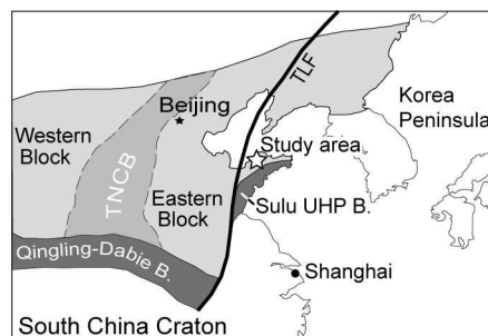
Figure 5.1: Tectonic sketch of eastern Asia with Jiaodong Peninsula location. TLF = Tan-Lu fault. TNCB=Trans-North China Belt.
