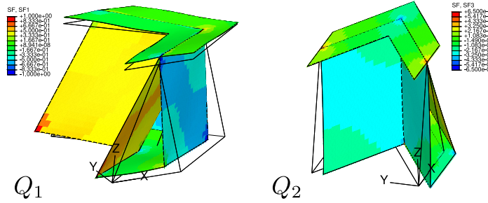
Figure 7.7: Deformed unit-cell under shear forces loading ( a_0/b_0 = 1.2 , t_f = 0.1 \text{ mm} , t_s = 1 \text{ mm} ). The contour plot displays local membrane stress n_{11}^{(Q)} for Q_1 loading and n_{12}^{(Q)} for Q_2 loading
