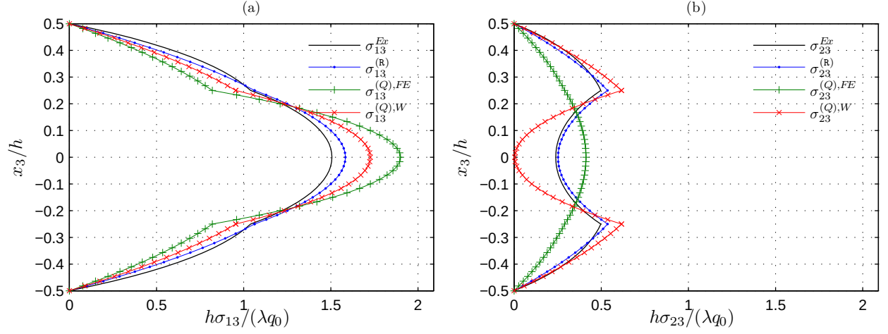
Figure 5.8: Normalized shear distribution in both directions at x_1 = 0 for a [30^\circ, -30^\circ]_s laminate, L/h = 4 , a) \sigma_{13} b) \sigma_{23} .
