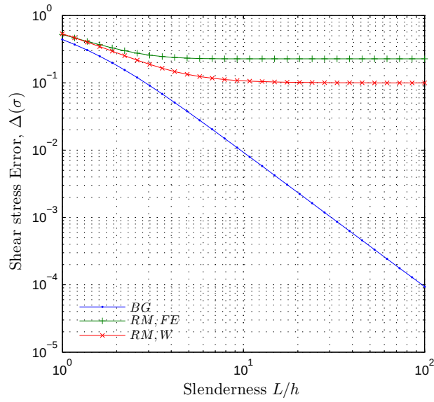
Figure 5.9: Shear stress distribution error versus slenderness ratio for a [30^\circ, -30^\circ]_s laminate
