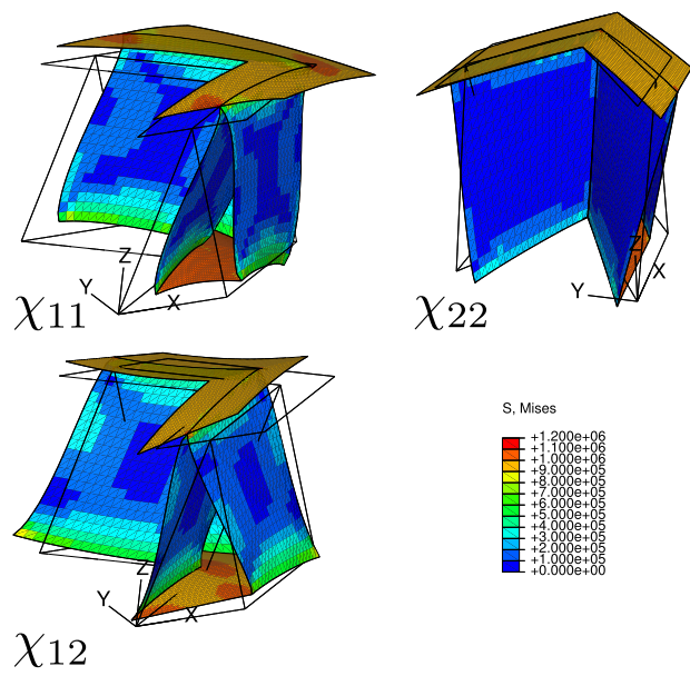
Figure 7.4: Deformed unit-cell under Curvature \chi loading ( a_0/b_0 = 1.2 , t_f = 0.1 \text{ mm} , t_s = 1 \text{ mm} ). The contour plot displays Von Mises stress.
