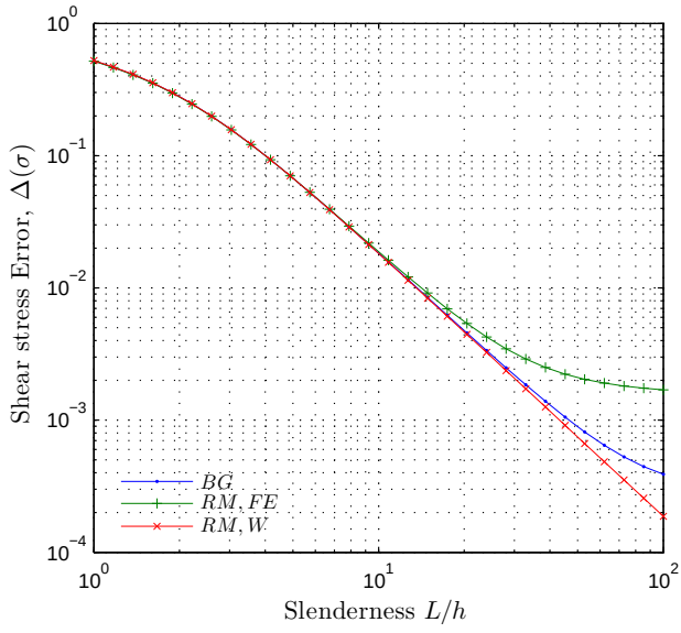
Figure 5.6: Shear stress distribution error versus slenderness ratio for a [0^\circ, 90^\circ] laminate, ( BG : Bending-Gradient, RM, FE : finite elements, RM, W :Whitney's distribution)
