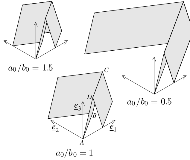
Figure 7.1: Chevron pattern investigated configurations
