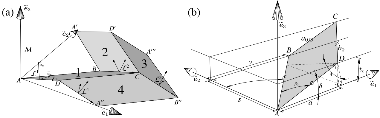
Figure 3.2: The four elementary faces of the pattern (a) and Face 1 orientation (b)
