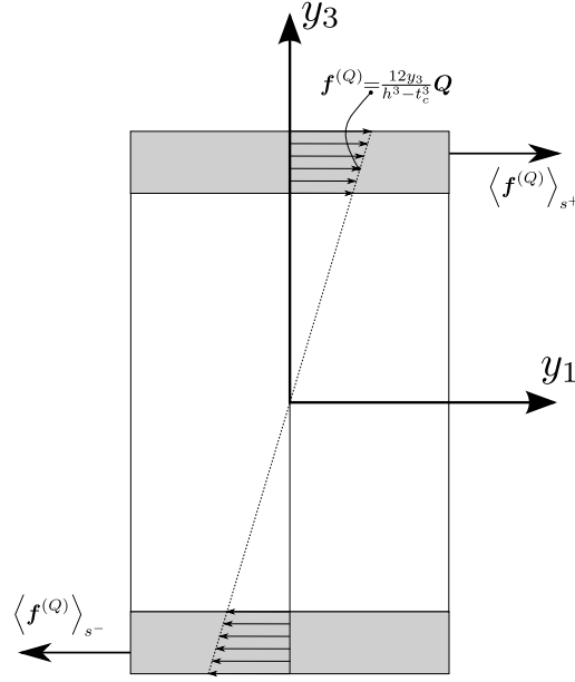
Figure 6.3: Shear force loading \mathbf{f}^{(Q)-} for a sandwich panel with thin skins
