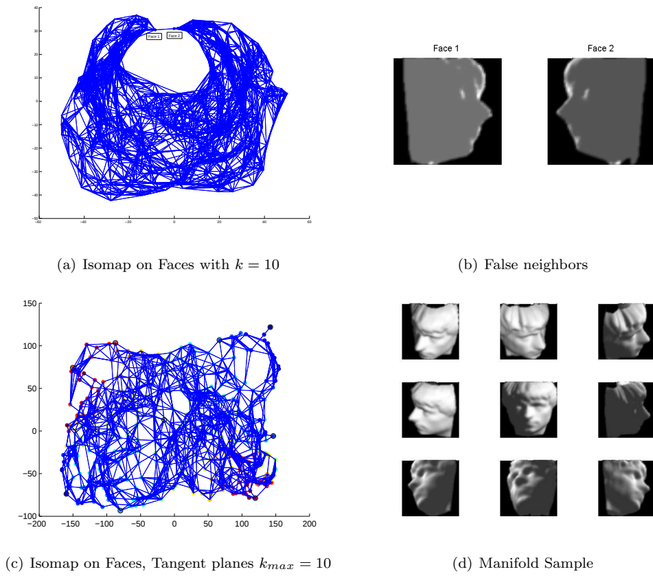
Figure 3.14: Illustration of the algorithm use in the faces datasets.
