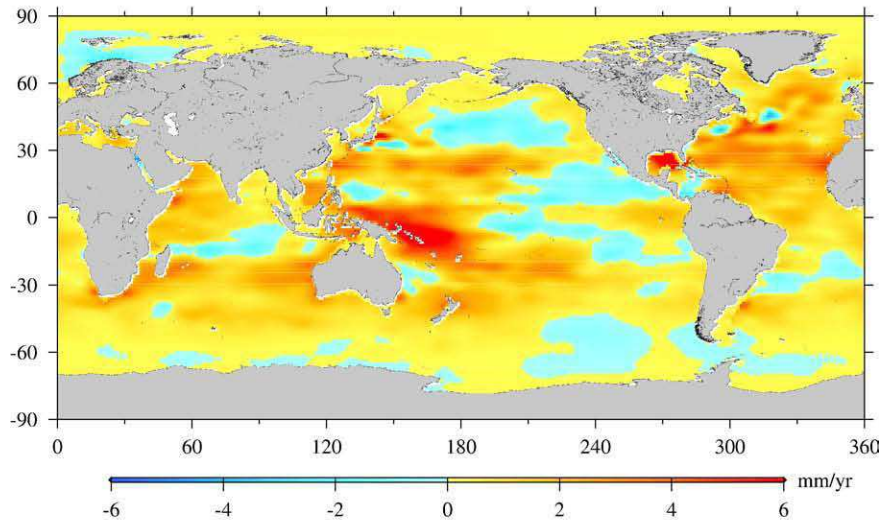
Reconstructed sea level trend map (1993-2003)
