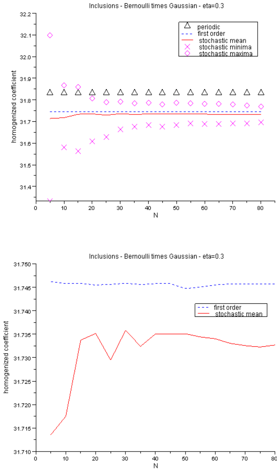
Figure 4.4: Inclusions - results for perturbation (4.116) and \eta = 0.3 . Above: complete results. Below: close-up on A_{\eta}^{*,N} and the first-order correction.
