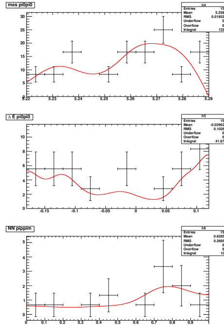
Figure B.5: K_S^0 K_L^0 K^{0*} B background for B^0 \rightarrow 2K_S^0(\pi^+\pi^-)K_S^0(\pi^0\pi^0) .
