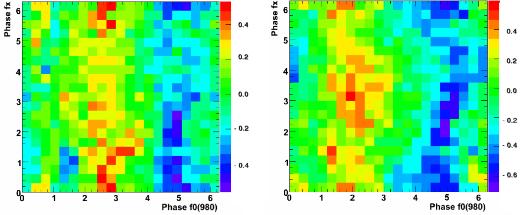
Figure 9.11: Two-dimensional scans of the phases of the f_0(980) and f_X(1500) resonances. For each scan point we generate 100 toy experiments and fit them. The plotted value is the difference between the average of the fitted value and the generated one, divided by the error on the average of the fitted value. This way we get an estimate of the bias in units of the error. The plot on the left (right) shows the bias of the fitted phase of the f_0(980) ( f_X(1500) ).
