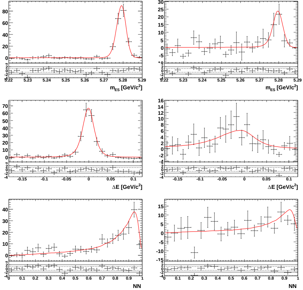
Figure 8.8: Signal sPlots of the discriminating variables for B^0 \rightarrow 3K_s^0(\pi^+\pi^-) on the left and for B^0 \rightarrow 2K_s^0(\pi^+\pi^-)K_s^0(\pi^0\pi^0) on the right. The first row shows the m_{ES} distribution, the second row the \Delta E distribution and the third one the NN output distribution.
