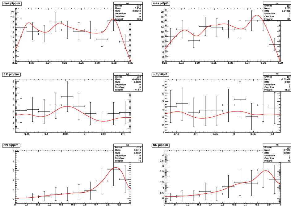
Figure B.3: K_s^0 K_s^0 K_L^0 B background for B^0 \rightarrow 3K_s^0(\pi^+\pi^-) (left) and B^0 \rightarrow 2K_s^0(\pi^+\pi^-)K_s^0(\pi^0\pi^0) (right).
