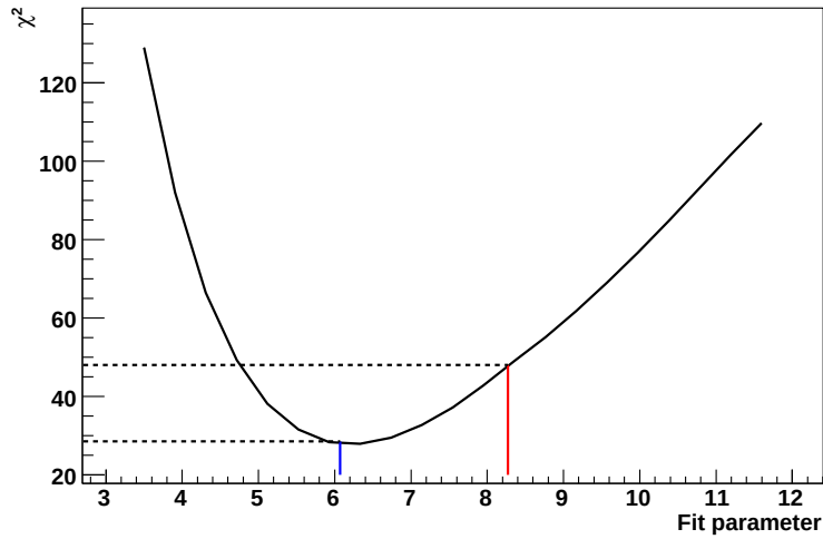
Figure 5.9: Scan of the \chi^2 for the fit parameter for 2 scale-corrected midplane modules. The blue line is the value for the scale-corrected midplane-module data points wrt the model fitted to non-midplane modules. The red line is the value of the fit parameter so that the minimum of the curve would correspond to the highest dose-value for the scale-corrected points.
