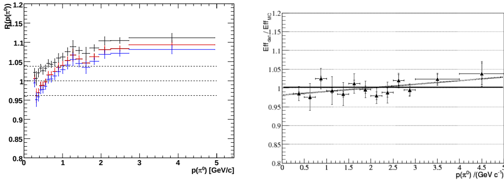
Figure 6.10: Double ratio as obtained in the present study (left) and in the previous study (right). The red points indicate the "raw" double ration, the black ones are corrected for the difference of the number of candidates between data and MC. The blue points give the simple ratio \frac{N_{K\pi\pi^0}(p_{\pi^0})|_{data}}{N_{K\pi\pi^0}(p_{\pi^0})|_{MC}} , where the MC yield has been scaled to luminosity. The dashed lines indicate the uncertainty from the branching fraction measurements.
