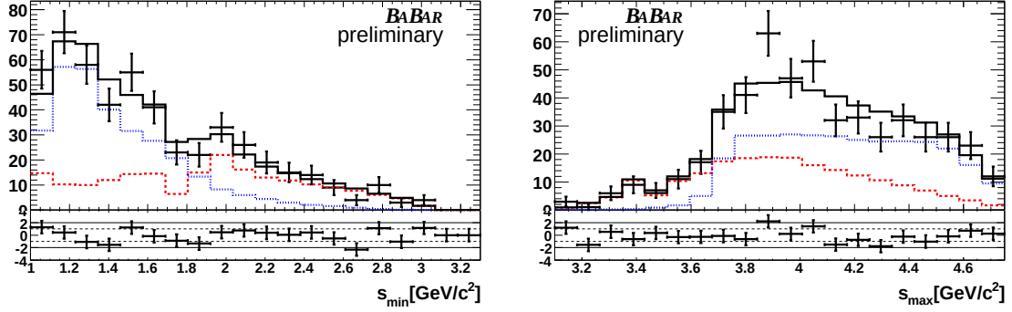
Figure 9.15: Projection plots of the s_{\min} (left) and s_{\max} (right). On-resonance data are shown as points with error bars while the dashed red (dotted blue) histogram represents the signal (continuum) components. The black histogram is the total PDF. Below each bin are shown the residuals, normalized in error units.
