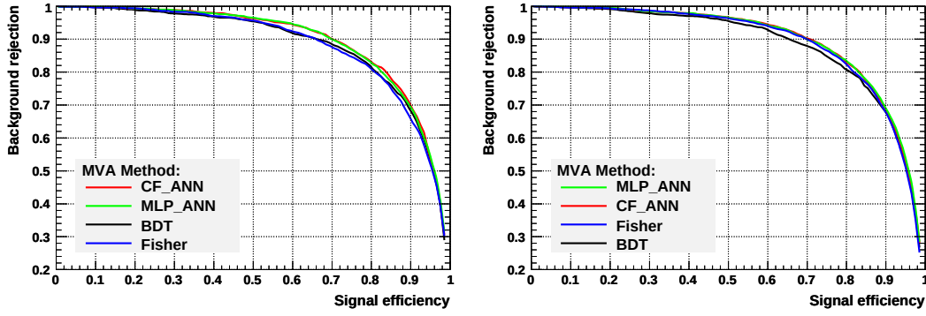
Figure 7.2: The background rejection over signal efficiency curves for B^0 \rightarrow K_s^0(\pi^+\pi^-)K_s^0(\pi^+\pi^-)K_s^0(\pi^+\pi^-) (left) and B^0 \rightarrow K_s^0(\pi^+\pi^-)K_s^0(\pi^+\pi^-)K_s^0(\pi^0\pi^0) (right) show that the CFMLpANN has the best discriminating power or is at least equally discriminating when comparing to other standard classifiers.
