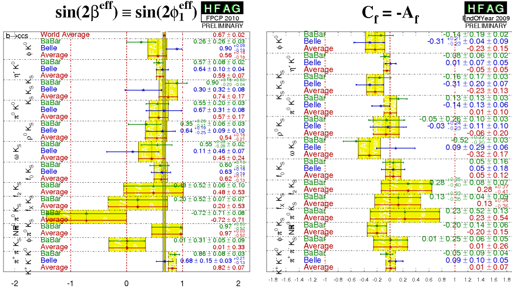
Figure 8.13: Compilation of \sin(2\beta_{\text{eff}}) and \mathcal{C} for penguin dominated decays by the HFAG group [15].
