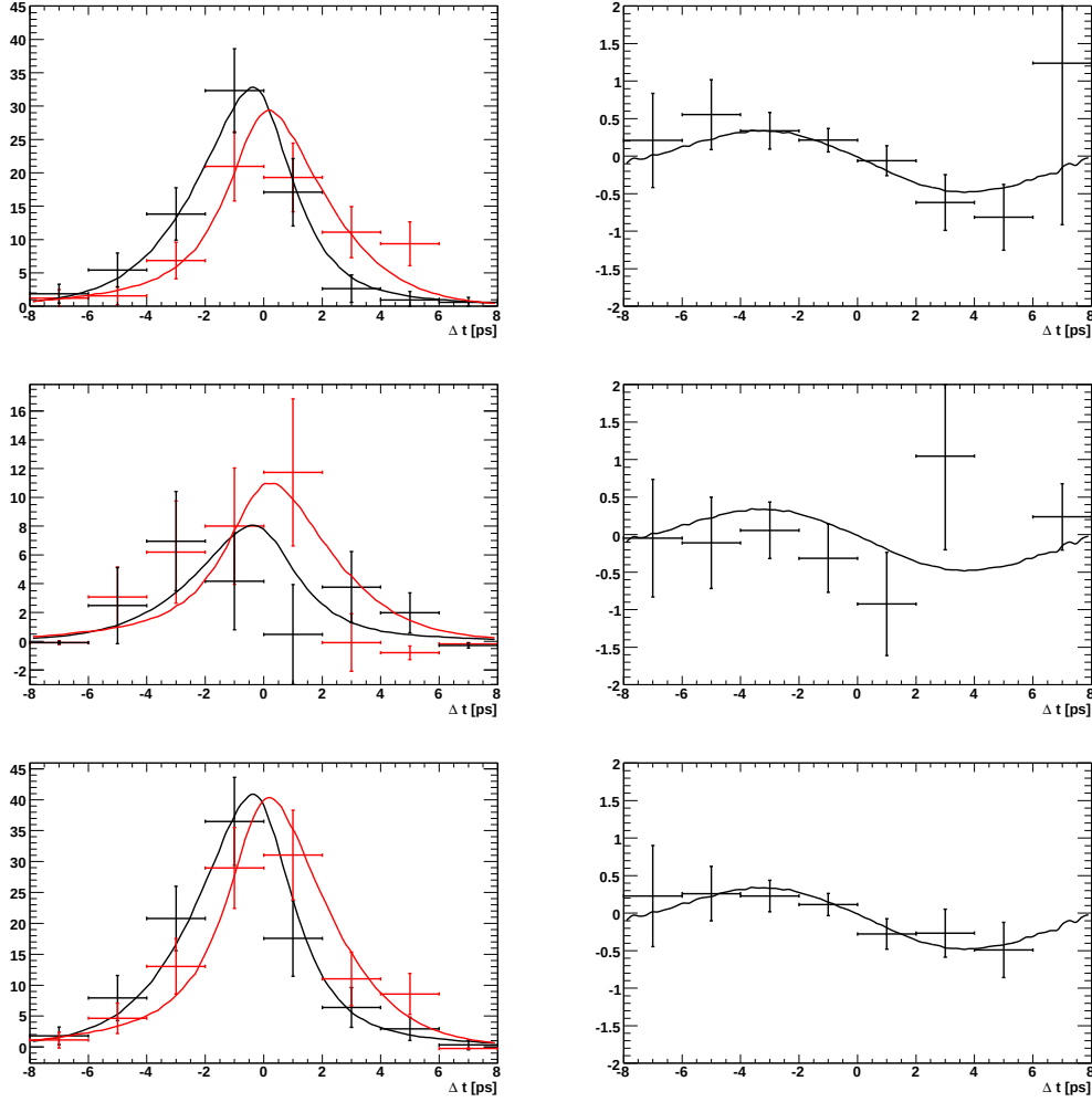
Figure 8.10: s\mathcal{P} lots for signal \Delta t . On the left are shown the proper-time distributions for signal B mesons tagged as B^0 in black and \bar{B}^0 in red, on the right are shown the time-dependent CP asymmetry distributions. The data points with error bars in the first row corresponds to B^0 \rightarrow 3K_s^0(\pi^+\pi^-) , in the second to B^0 \rightarrow 2K_s^0(\pi^+\pi^-)K_s^0(\pi^0\pi^0) and in the third to both, the smooth lines correspond to the combined fit result in all cases.
