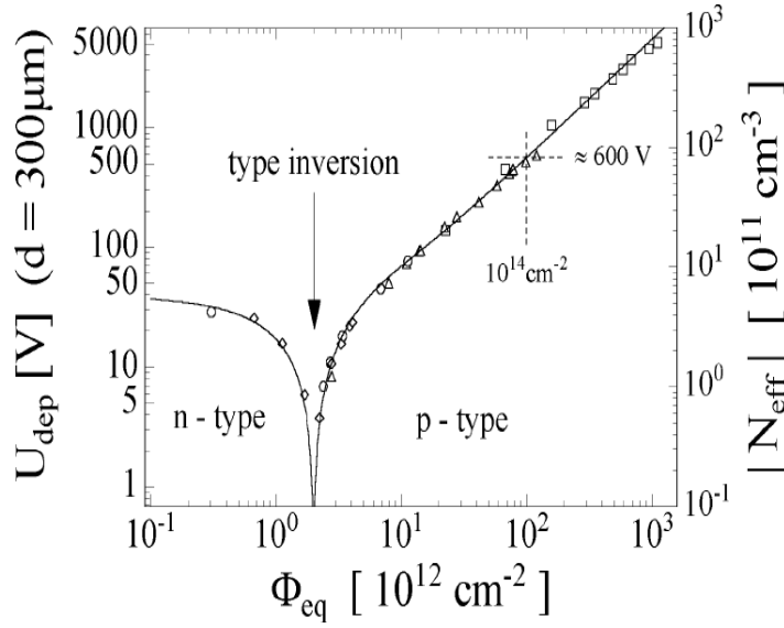
Figure 5.3: Depletion voltage V_{\text{dep}} and effective doping concentration N_{\text{eff}} as function of 1 MeV neutron equivalent fluence measured directly after irradiation. Plot taken from [42].
