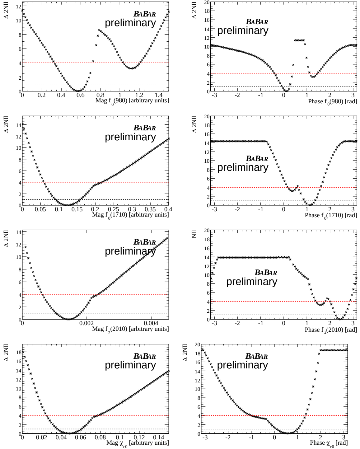
Figure 9.13: Likelihood scans of the magnitudes (left) and phases (right) for all resonances (from top to bottom: f_0(980) , f_0(1710) , f_2(2010) , \chi_{c0} ). The black (red) dashed line indicates the one (two) standard deviation level.
