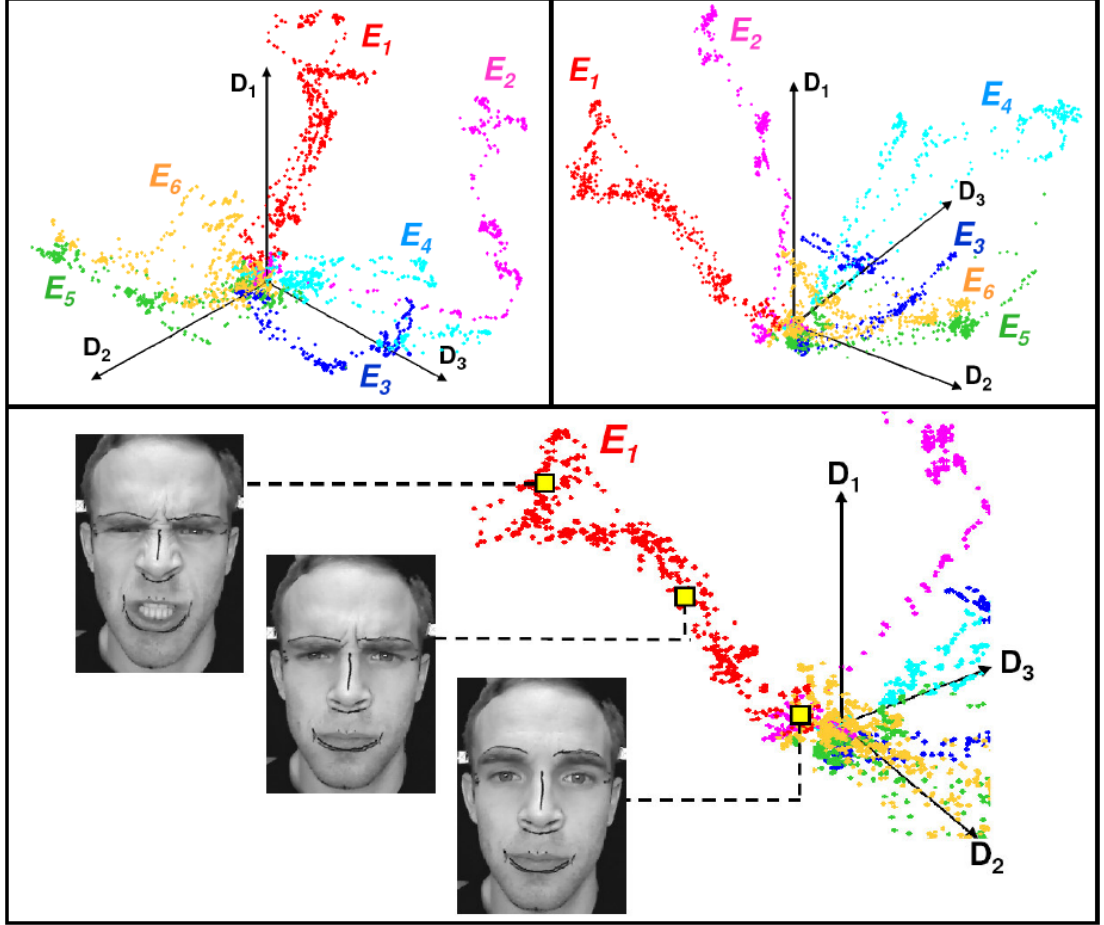
Figure 3.6: Top: two different views of the database samples distribution on the first three dimensions of the appearance space. Bottom: the expressions of varying intensities are concentrated on dominant directions in space. Neutral expressions are located in the center, and extreme expressions on the edge of the point cloud.
