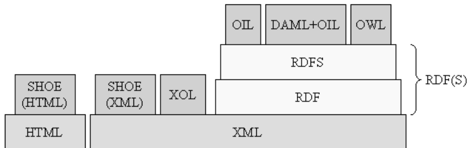
FIGURE A.3: Ontology markup languages
