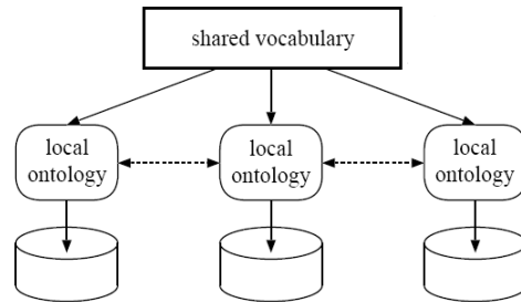
FIGURE 2.3: Hybrid Ontology Approach
