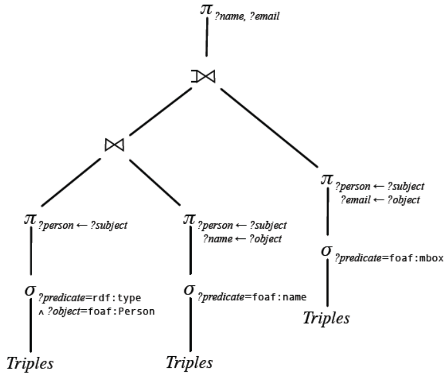
FIGURE G.1: Relational Tree for Cyganiak's Relational Algebra for SPARQL
