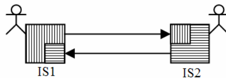
FIGURE 1.1: Database-Translation approach
