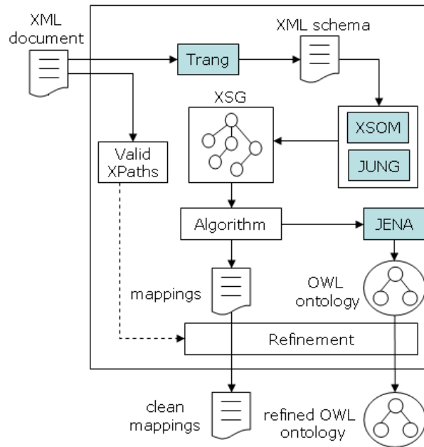
FIGURE 10.8: X2OWL implementation
