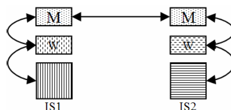
FIGURE 1.6: Mediator-wrapper approach
