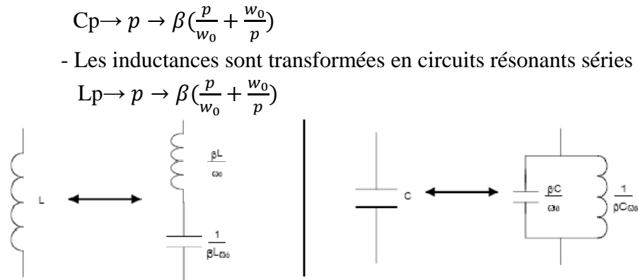
Fig E. 4. Transformation passe-bas passe-bande
