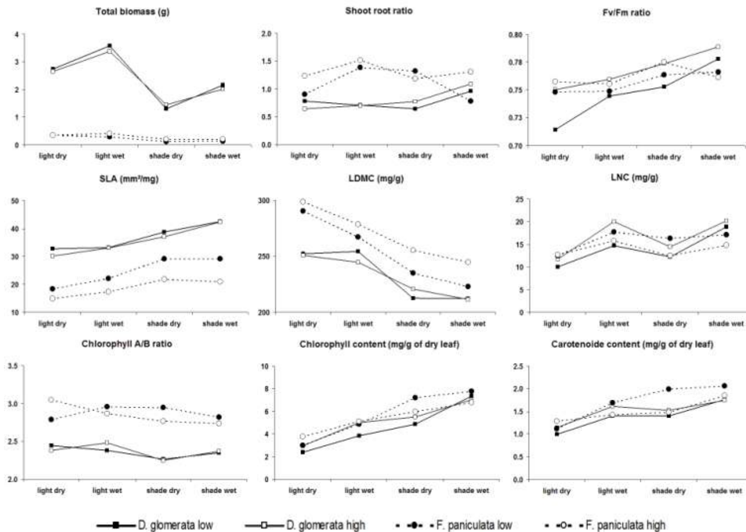
Figure 1 : Reaction norms of the traits showing the population means for each species in the four treatments. Solid lines represent Dactylis glomerata (open square: high population, solid square: low population). Dashed lines represent Festuca paniculata (open circle: high population, solid circle: low population).
