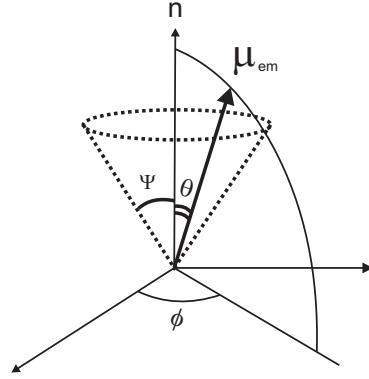
Figure 3.7: Wobbling-in-cone model [69].
