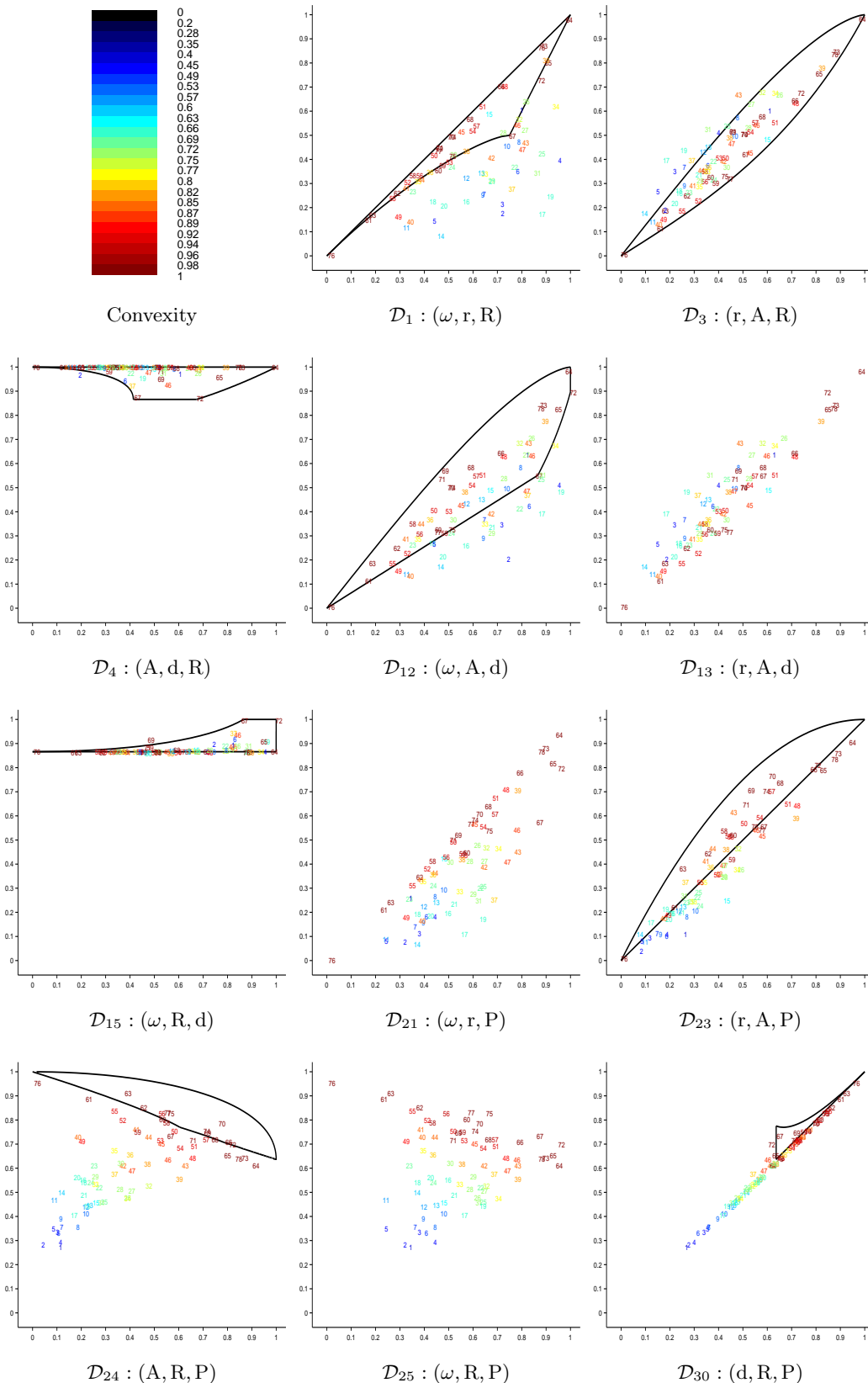
FIG. 4.37 – Family \mathcal{F}_1^{disc} of discretized simply connected compact sets mapped into eleven shape diagrams (chosen according to the results synthetized at the end of the part II of this study [RDP10b]).
