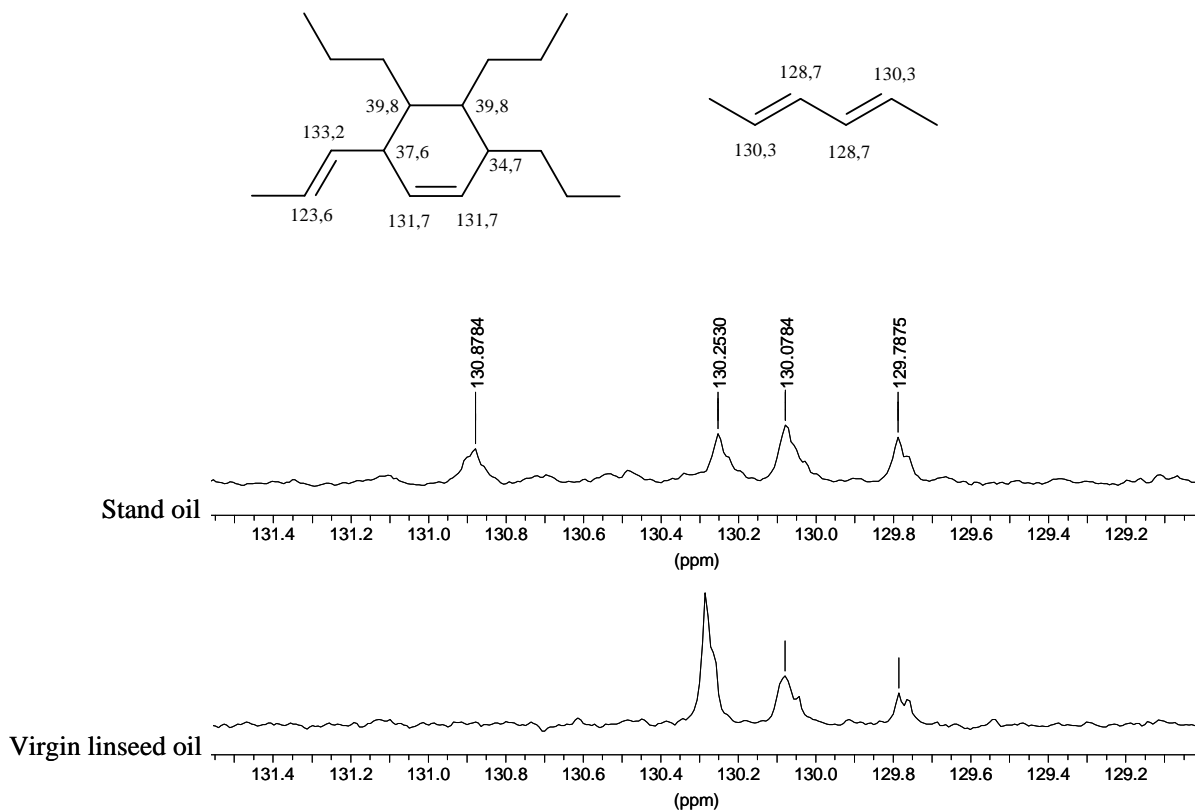
Figure 7: Evolution of ^{13}\text{C} NMR spectrum of linseed oil after 6 hours at 300^\circ\text{C} in the spectral range 30-34 ppm and 129-132 ppm.
