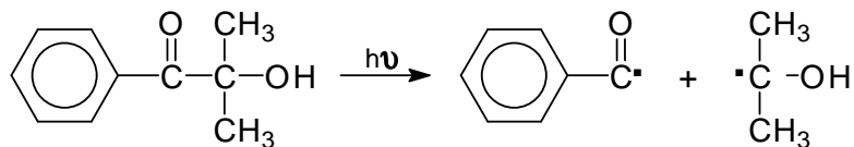
Figure 42 : Photolyse du 2-hydroxy-2-méthyl-1-phényl-propan-1-one (DAROCUR 1173 ® - Ciba Geigy Specialties)
