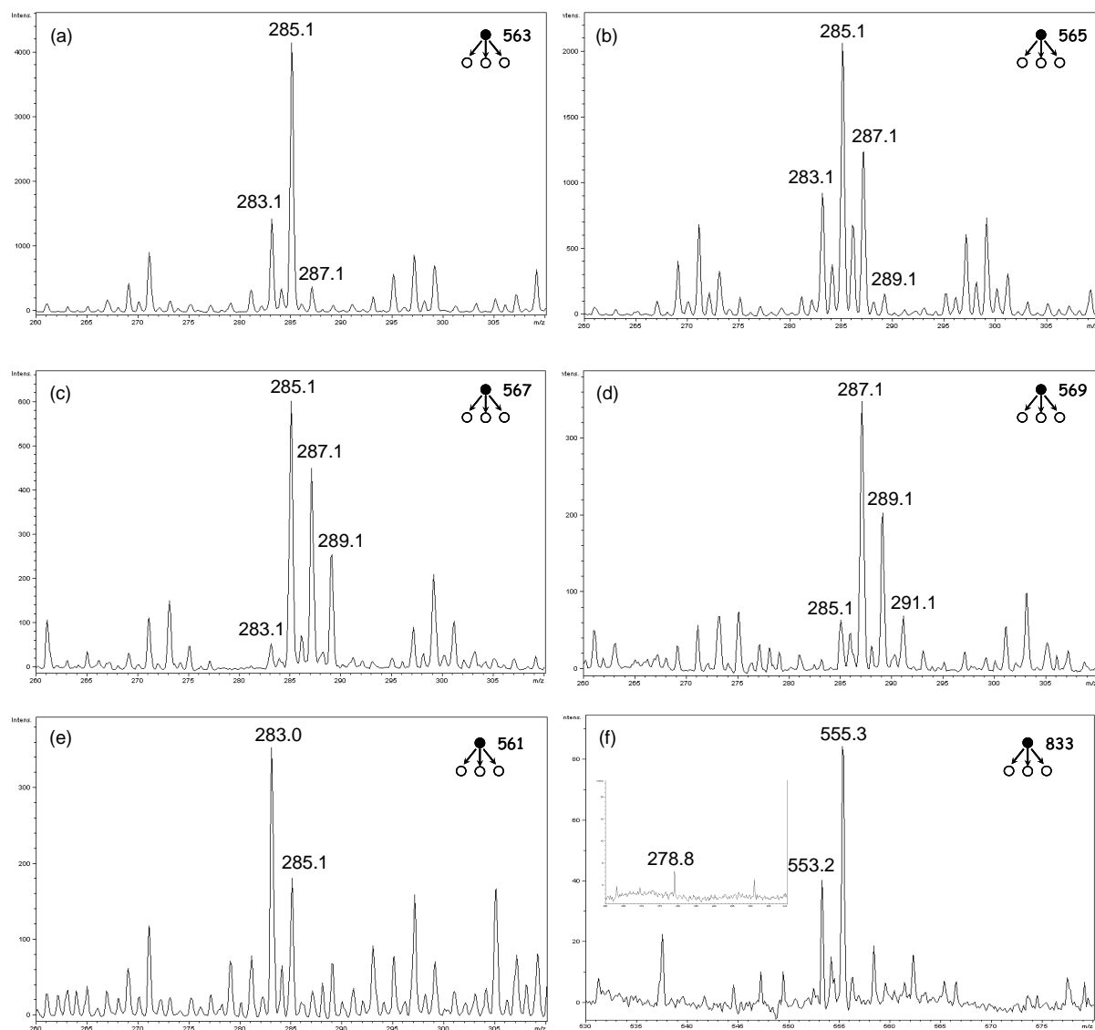
Figure 9: MS/MS spectrum of ions at m/z 563 (a), 565 (b), 567 (c), 569 (d), 561 (e) and 833 (f) present in the saponified stand linseed oil.
