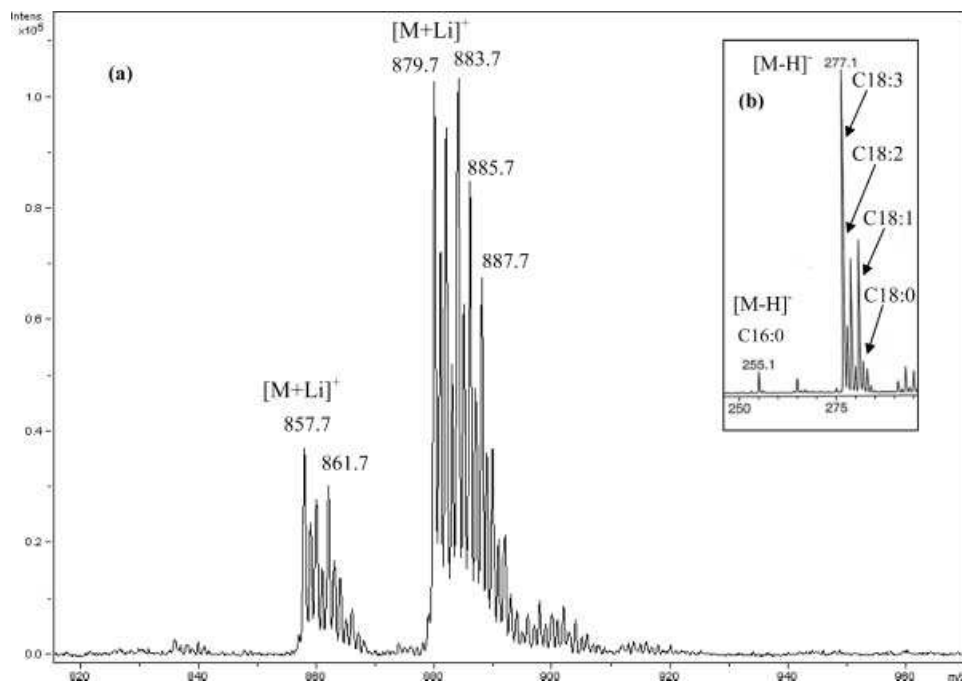
Figure 1. (a) Positive ESI-MS spectrum of linseed oil (batch 2). Direct flow injection of 10 ng/ \mu\text{L} solutions of oil containing aqueous LiI (1 mmol/L) permits the detection of [\text{M}+\text{Li}]^+ adducts. (b) The inset corresponds to the negative ESI-MS spectrum of saponified linseed oil: deprotonated molecules of constitutive palmitic, linolenic, linoleic, oleic and stearic acids are detected at m/z 255, 277, 279, 281 and 283, respectively.
