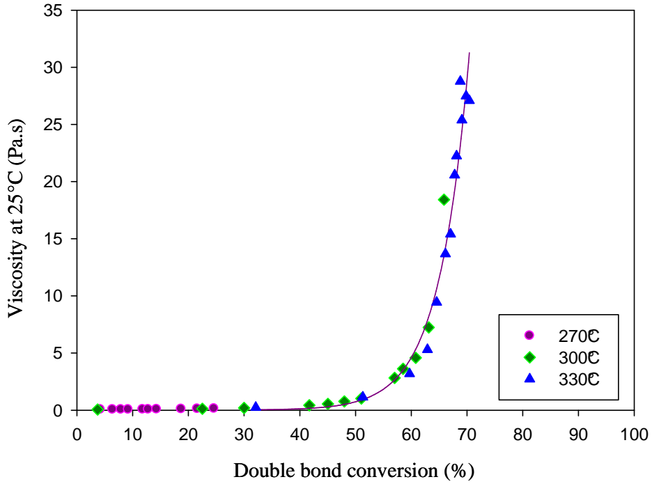
Figure 4: Evolution of the stand oil viscosity as a function of double bond conversion: (●): T = 270°C; (◆): T = 300°C; (▲): T = 330°C.
