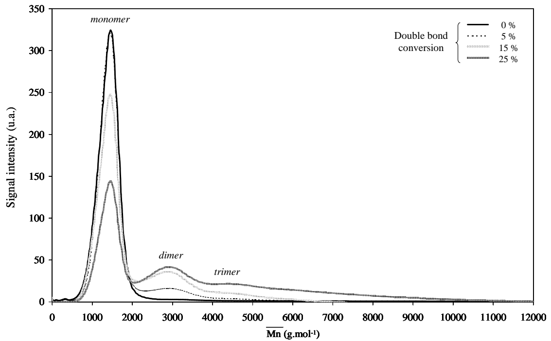
Figure 5: SEC chromatograms of linseed oil versus double bond conversion.
