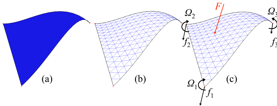
Figure 8.2: (a) The triangle formed by the three vertices of the shell has been recursively subdivided 3 times and the deflection of each new vertex was computed according to the same deflection function used in our shell FEM. (b) Sampling the actual surface of the shell allows more accurate rendering and collision detection. (c) The shape function is used to distribute an external force F onto the triangle nodes.
