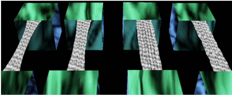
Figure 7.3: A 400% stretched fabric square with various Poisson's ratio. Image courtesy of Volino and Magnenat-Thalmann (1997) .
