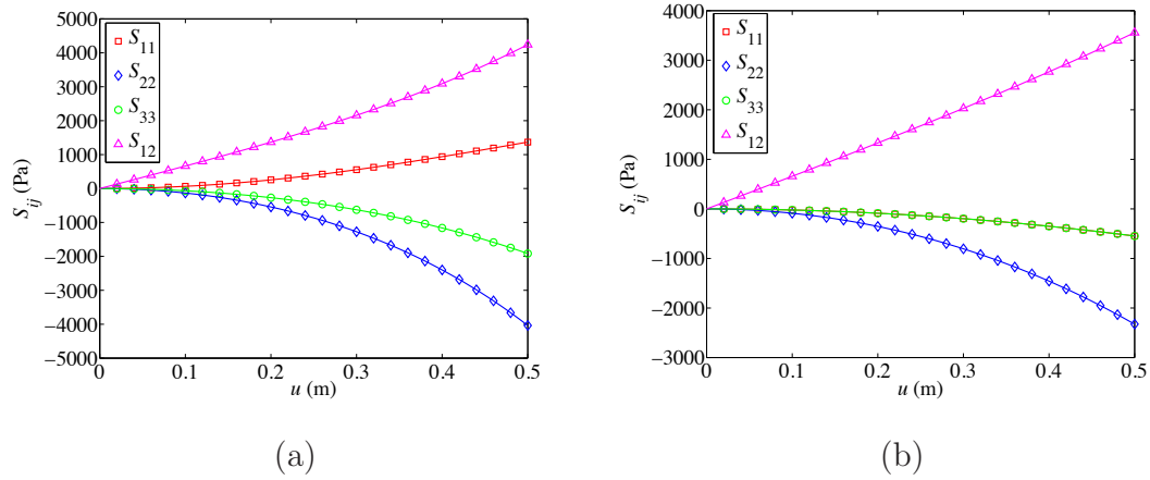
Figure 6.3: Instantaneous stress curves for pure shear deformation of (a) the anisotropic model compared with those of (b) an isotropic model. Solid lines correspond to the analytical solution, while markers indicate the FE solution.
