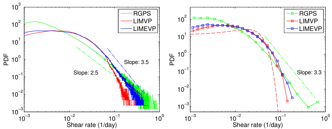
FIG. 2.8: PDF of shear rates for the period January-March 1997, from RGPS observations (green), LIMVP experiment (red) and LIMEVP (blue), at scales of \sim 10\text{km} (left panel) and \sim 100\text{km} (right panel). The green and blue dashed lines indicate, respectively, the slope of the RGPS and LIMEVP distributions. On the right panel, the red dashed line is the Gaussian distribution of same mean and standard deviation as the LIMVP distribution.
