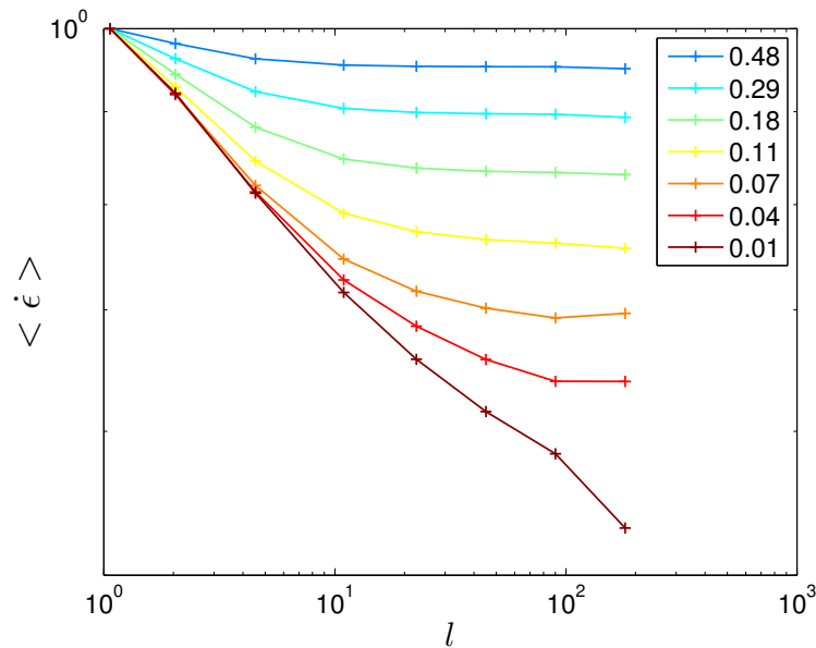
FIG. 3.15: Mean total deformation rate as a function of the spatial scale l and of the control parameter \Delta , for the random mesh under strain control ( H_1 -range, L = 128 ). Deformation rates are normalized at scale l = 1 .
