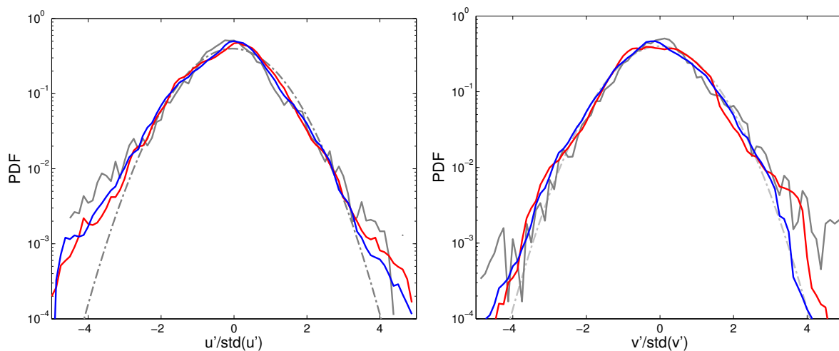
FIG. 2.4: PDFs of the two components of velocity fluctuations of 12-hourly velocity ( u' , left panel and v' right panel), normalized by their standard deviation (buoys measurements : grey, model, LIMVP : red, LIMEVP : blue) and the corresponding Gaussian distribution ( \mu = 0; \sigma = 1 , dashed line). The standard deviations are as follows : std(u'_{buoys}) = 3.11 , std(v'_{buoys}) = 3.28 , std(u'_{LIMVP}) = 6.74 , std(v'_{LIMVP}) = 6.05 , std(u'_{LIMEVP}) = 6.13 , std(v'_{LIMEVP}) = 5.53 .
