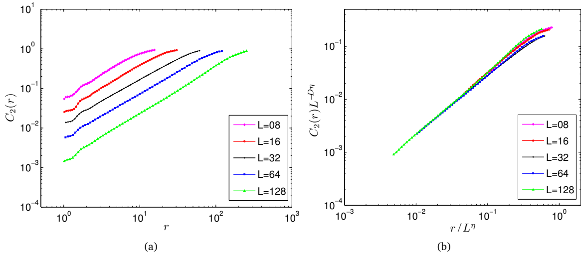
FIG. 3.10: (a) The correlation integral C_2(r) of damage events near peak load ( \Delta < 10^{-2} ) for different system sizes, for the random mesh under strain control ( H_1 -range). (b) Data collapse analysis of the correlation integrals, the values used for the exponents are D = 1.15 and \eta = 1.1 .
