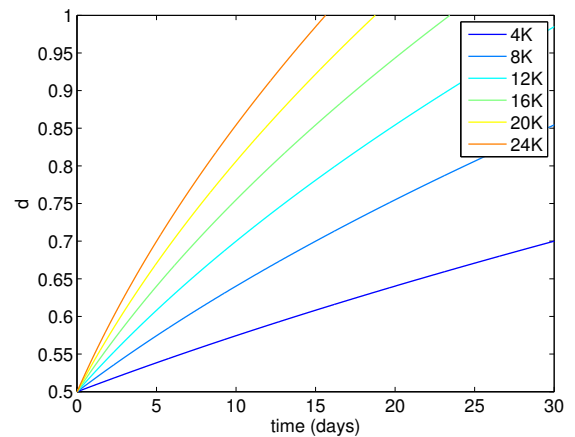
FIG. 5.5: Evolution of d due to healing as a function of time for different temperatures T_f - T_a (K) and an initial value of d(0) = 0.5 ( \beta = 10^3 \text{ day.K}^{-1} ).
