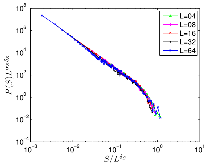
FIG. 3.5: Data collapse of the distributions of avalanche size S for the random mesh under strain control, \alpha_S = 2.8 and \delta_S = 1.3 ( H_2 -range).
