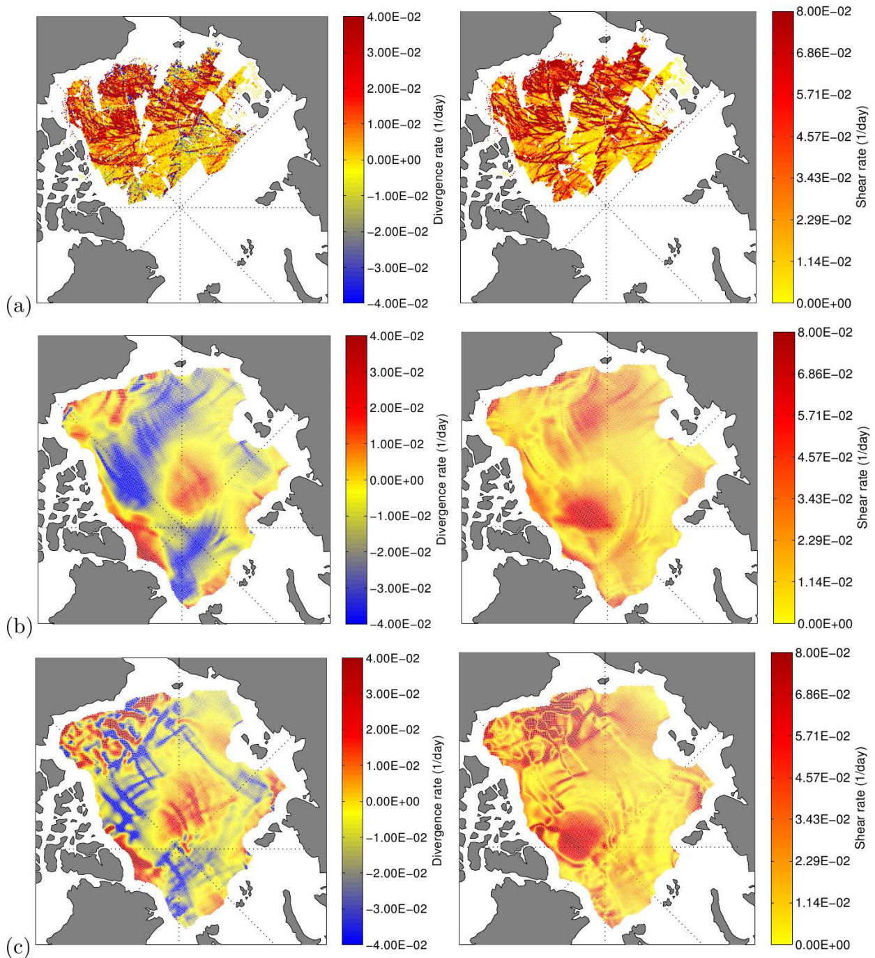
FIG. 2.5: Divergence and shear rate fields ( /\text{day} ), from RGPS observations (a), LIMVP (b) and LIMEVP (c), for the period 16-18 January 1997.
