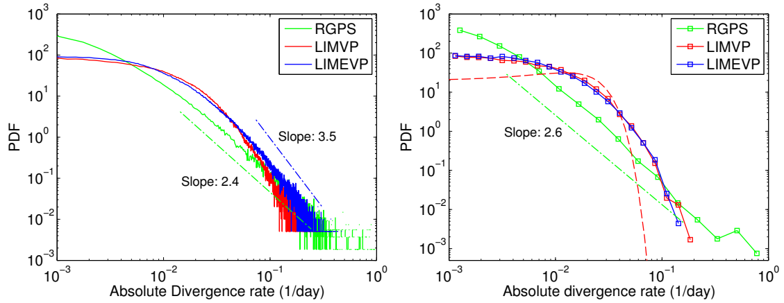
FIG. 2.7: PDF of absolute value of divergence rates for the period January-March 1997, from RGPS observations (green), LIMVP experiment (red) and LIMEVP (blue), at scales of \sim 10\text{km} (left panel) and \sim 100\text{km} (right panel). The green and blue dashed lines indicate, respectively, the slope of the RGPS and LIMEVP distributions. On the right panel, the red dashed line is the Gaussian distribution of same mean and standard deviation as the LIMVP distribution.
