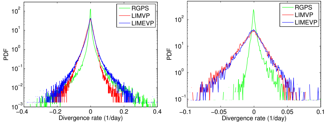
FIG. 2.6: PDF of divergence rates for the period January-March 1997, from RGPS observations (green), LIMVP experiment (red) and LIMEVP (blue), at scales of \sim 10\text{km} (left panel) and \sim 100\text{km} (right panel).
