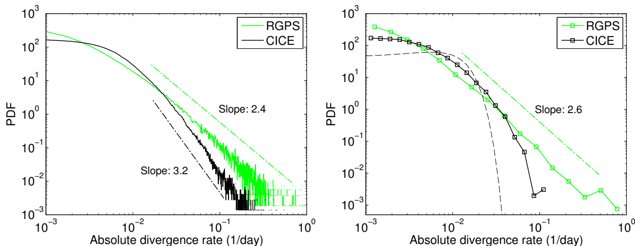
FIG. 2.9: PDF of absolute value of divergence rates from the CICE simulation (period January-March 1987) and from RGPS observations (period January-March 1997), at scales of \sim 10km (left panel) and \sim 100km (right panel). On the right panel, the black dashed line is the Gaussian distribution of same mean and standard deviation as the CICE distribution.
