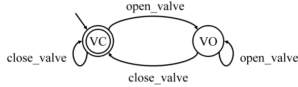
Figure 2.3: Automaton modeling a valve
