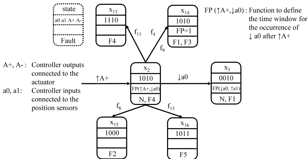
Figure 2.10: Part of a diagnoser from (Philippot, 2006)
