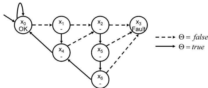
Figure 6.15: Tolerance specification for the case study system
