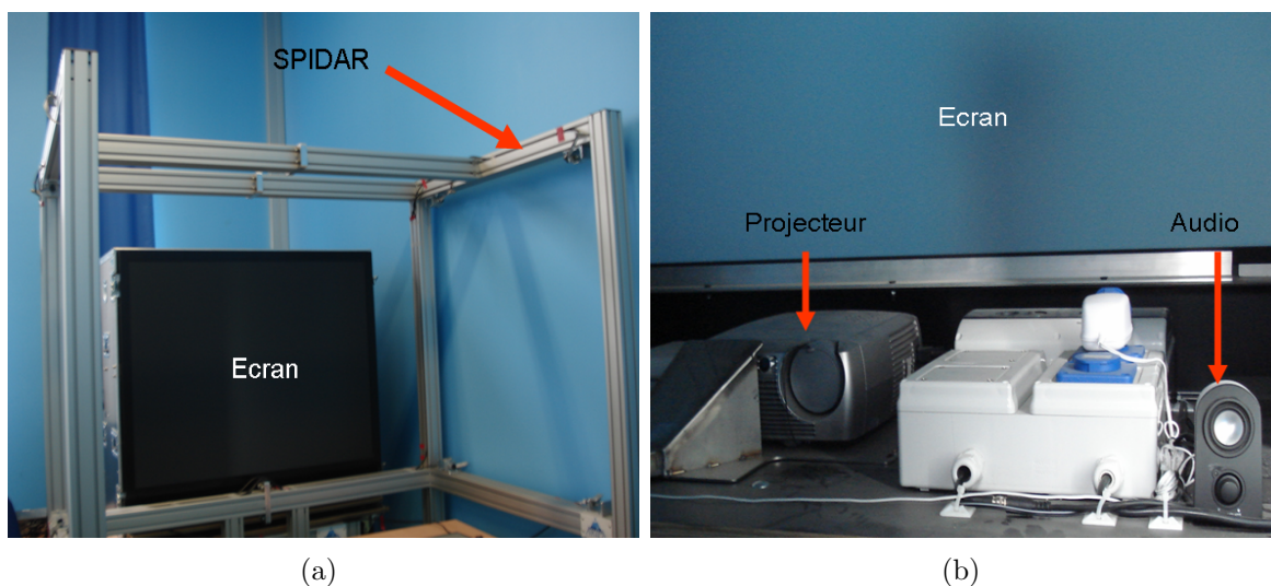
Figure 5.18: The mobile platform of Evr@ (a) external view (b) internal view
