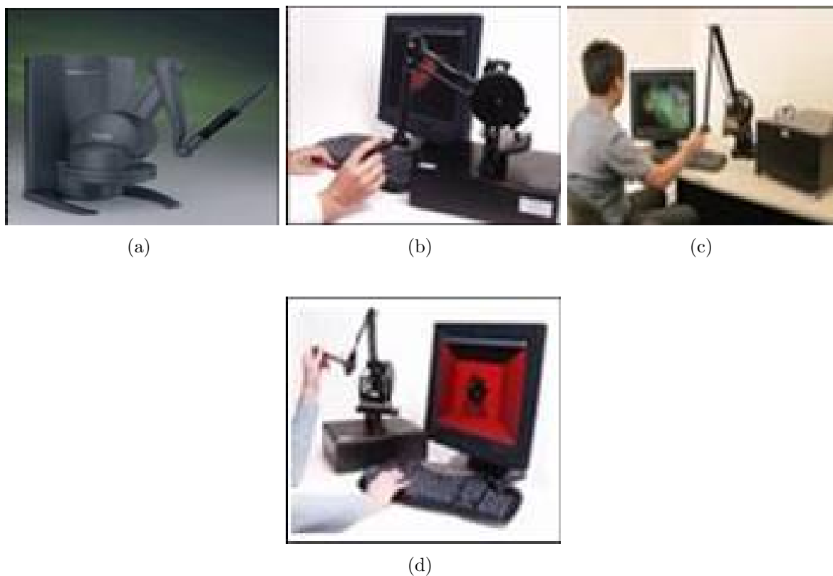
Figure 1.6: (a) Phantom desktop TM , (b) Phantom Premium TM 1.5/6 DOF, (c) Phantom Premium TM 3.0/6 DOF (d), and Phantom Premium TM 1.5/3 DOF (adopted from (SensAble, 2010))
