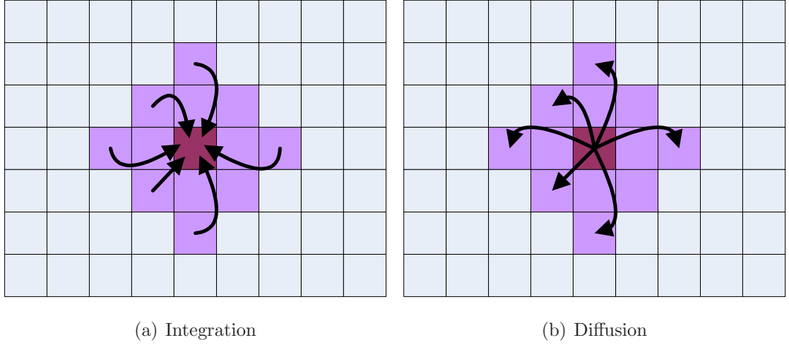
Figure 6.4 MRFs update with integration and with diffusion. With integration, the site s is updated with the neighborhood \eta_s . With diffusion, the neighborhood is updated with the local information at site s . Integration and diffusion are equivalent in terms of convergence.
