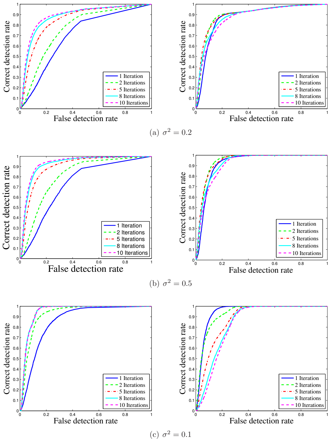
Figure 7.4 ROC curves for the stochastic clustering algorithm and for abnormal behavior detection based on probability density p(r|\Theta) for different values of neighborhood variance. Left column : Euclidian distance ABD-based; Right column : Mahalanobis distance ABD-based.
