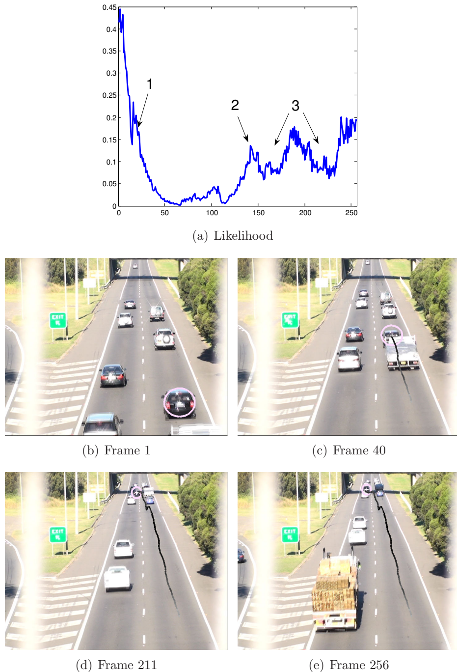
Figure 6.9 Vehicle tracking through large spatio-temporal occlusion. (a) The likelihood shows the total occlusion of the object (1→2), the recovery of the track (2) and distraction by visually similar objects and shadows (3). (b) Tracking initialization. (c) Tracking through partial occlusion. (d) and (e) Tracking recovery.
