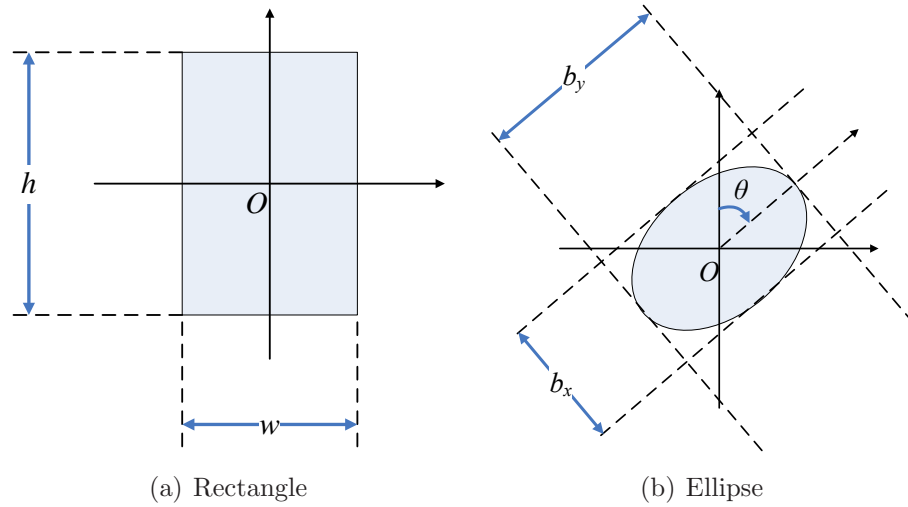
Figure 2.2 Example of rectangular and elliptic shapes with their nomenclature. The shapes are defined by a reduced number of parameters: 3 for the rectangle; 4 for the ellipse.
