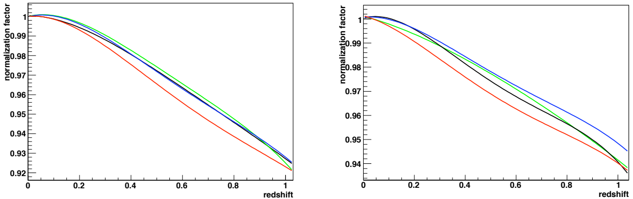
(a) The normalization factor for the galaxy-galaxy lensing (b) The normalization factor for the TF/FJ relations for the 4 different fields.
