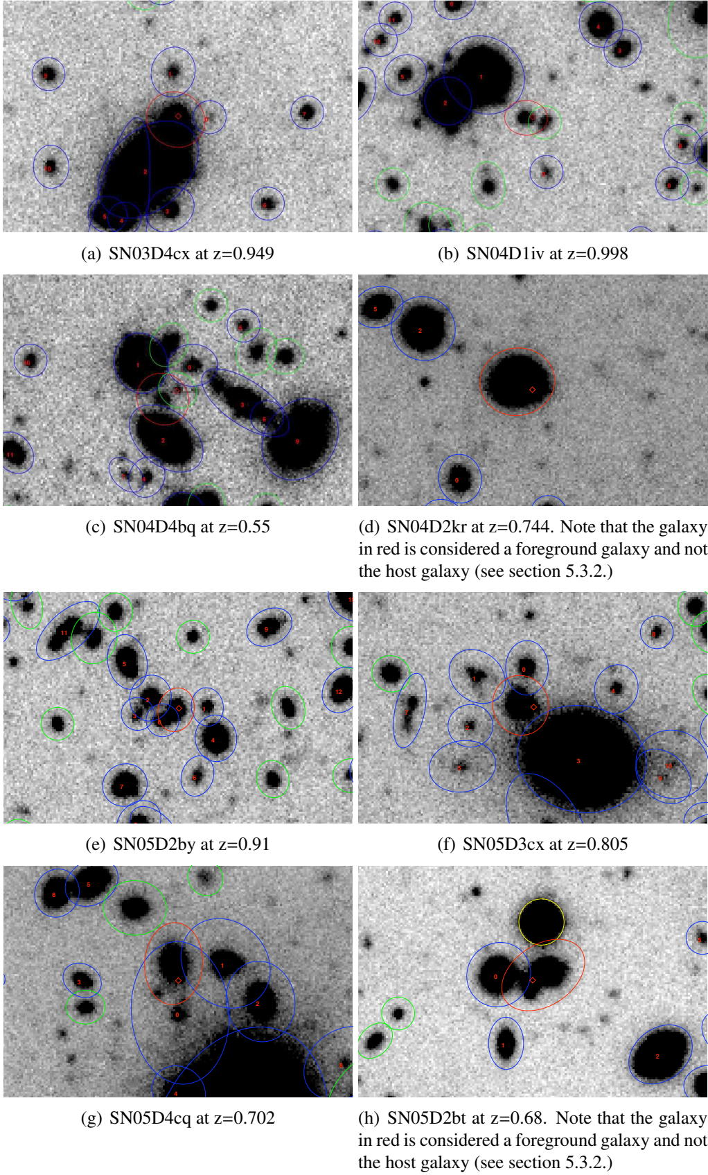
Figure 6.8: The most magnified supernova in the SNLS 3-year data set. In red: the supernova and the host galaxy. In blue: foreground galaxies. In green: background galaxies. In yellow: stars or saturated objects.
