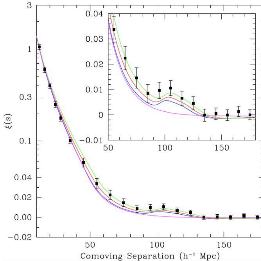
Figure 1.5: The two point correlation function for 46,748 galaxies out to a redshift of z = 0.47 covering 3816 square degrees of the sky measured by the SDSS team. The black dots are the data and the lines correspond to different models with different fractions of matter. The magenta line corresponds to a pure CDM universe. The small bump in the plot is the signature of BAO and is present at the characteristic scale \sim 100h^{-1}\text{Mpc} . Note that for a pure CDM universe, the BAO signature is not present. Credit: Eisenstein et al. (2005)
