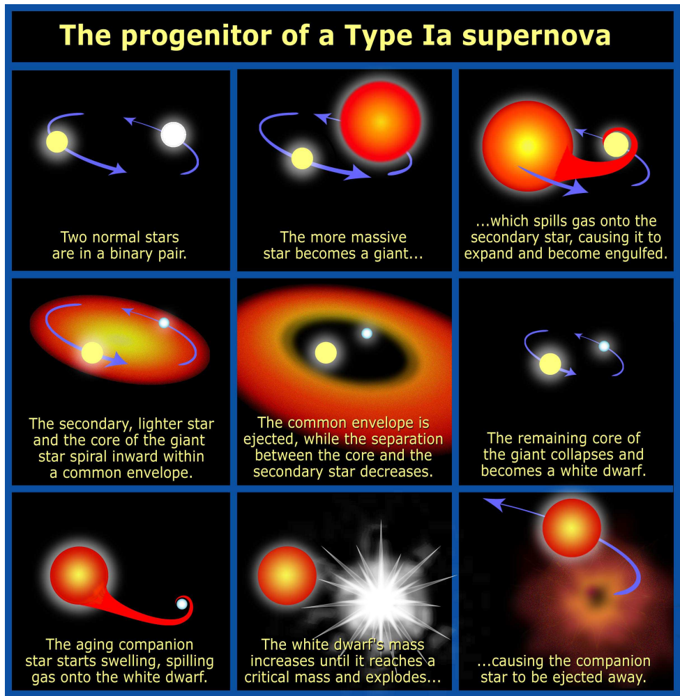
Figure 2.5: The progenitor of a Type Ia Supernova (Illustration credit: NASA, ESA, and A. Field (STScI))
