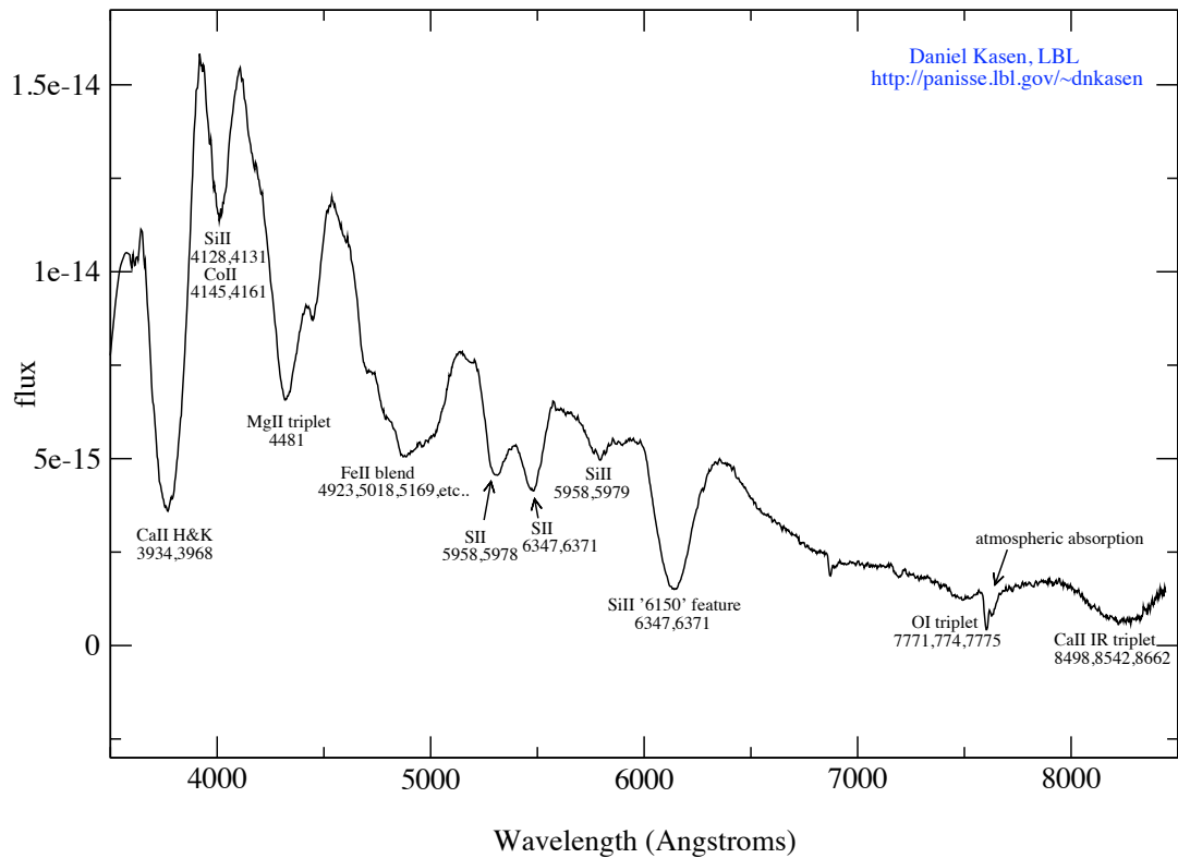
Figure 2.2: A typical SN Ia spectrum near maximum light showing the different absorption features. Credit: Daniel Kasen, LBL.
