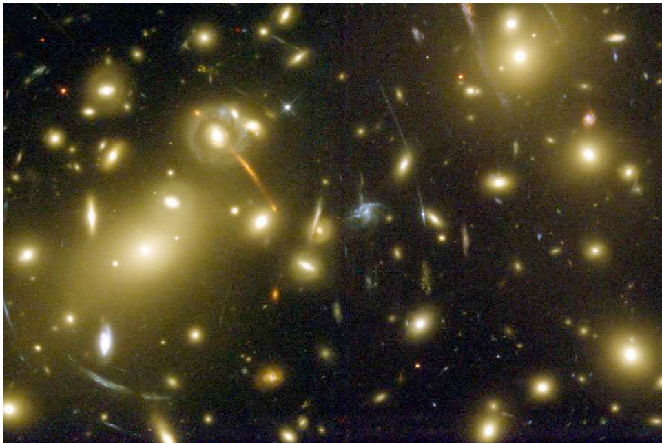
Figure 1.6: An image of the galaxy cluster Abel 2218 from the Hubble telescope where arcs and multiple images are present. Credits: NASA, Andrew Fruchter and the ERO team.
