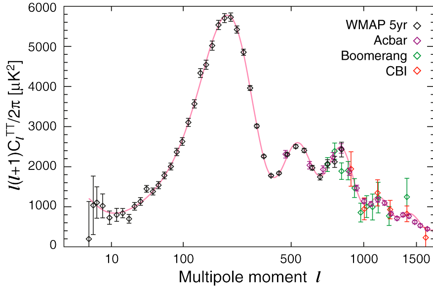
Figure 1.3: This figure illustrates the angular size of the observed temperature fluctuations. The large first peak corresponds to the maximum angular correlation in the CMB map. Credit: Nolta et al. (2009)
