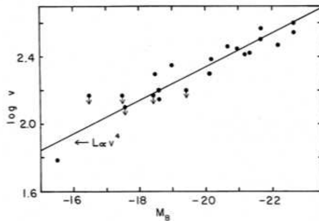
Figure 4.9: The original relation from Faber & Jackson (1976). Velocity dispersions versus absolute magnitude in the B-band. Credit: Faber & Jackson (1976)
