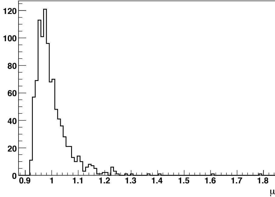
Figure 5.29: The magnification distribution for source positions at z=1 which peaks at a value slightly below one and presents a high magnification tail
