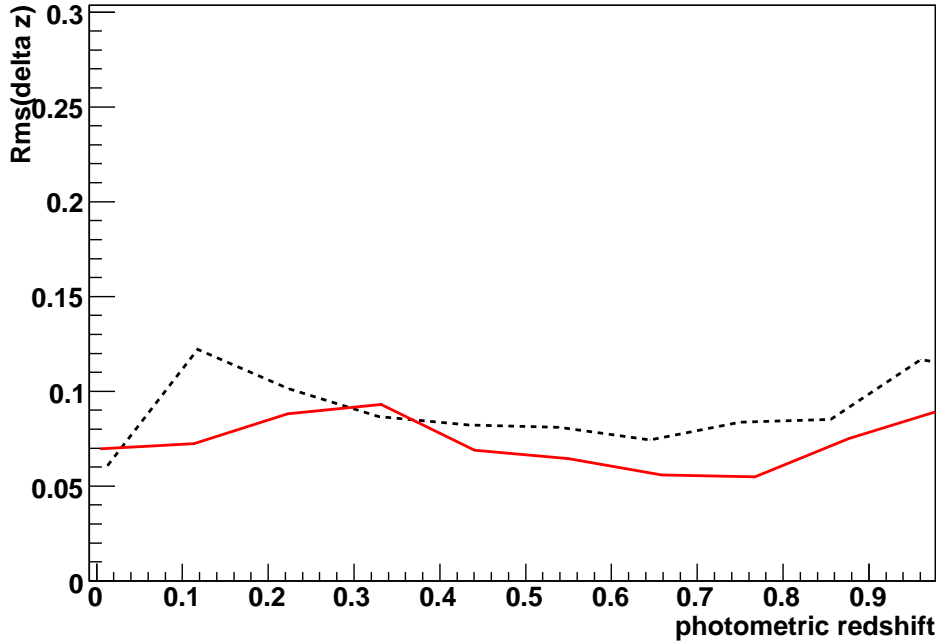
Figure 5.26: The rms of the z (photometric-spectroscopic(VVDS)) as a function of photo- z (in dotted black). The uncertainty obtained on the photo- z using Monte Carlo simulations (in solid red).
