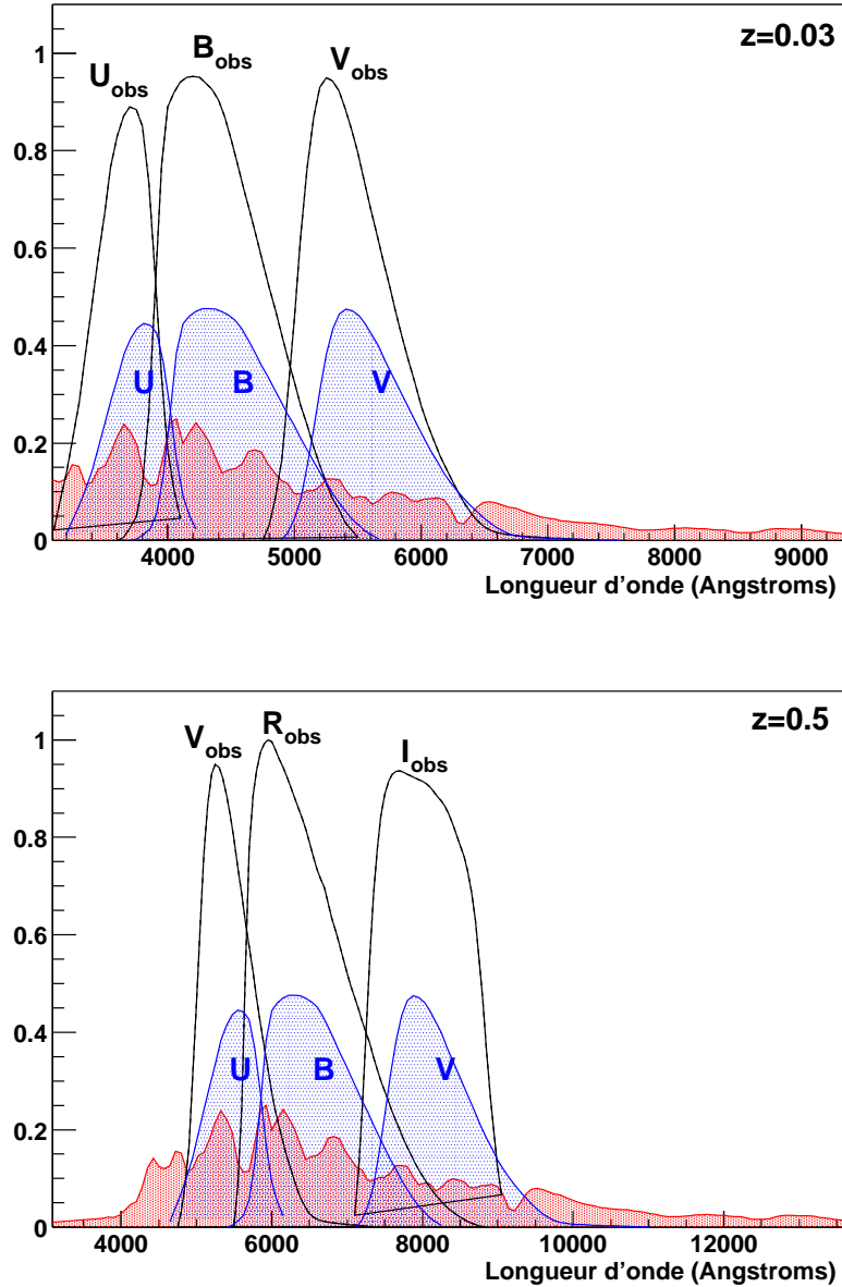
Figure 2.4: The spectrum of a supernova at z=0.03 (top panel) and z=0.5 (bottom panel). In blue, rest-frame bands. In black observational bands. The rest-frame B-band emission of the SN which can be measured with the B-band for a nearby SN but must be measured in the R-band for a redshifted SN. Credit: Guide (2005)
