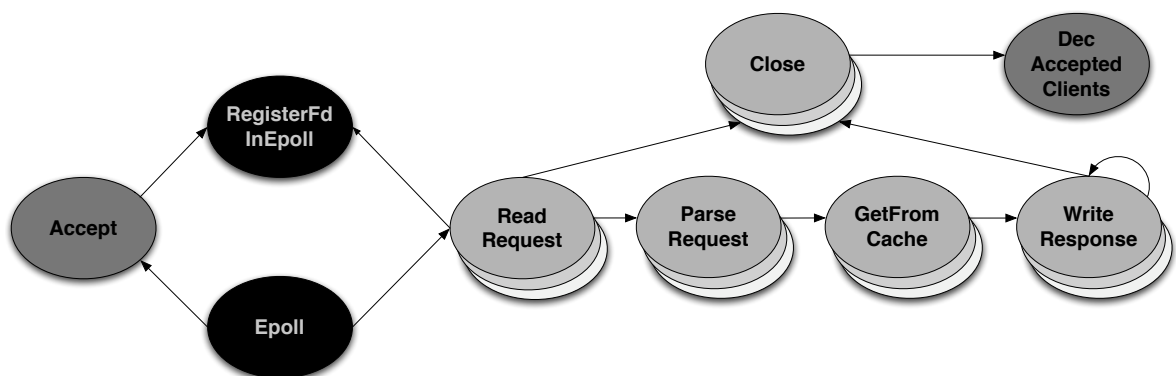
Figure 5.9 – Architecture du serveur Web SWS.
