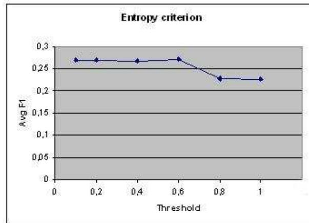
Figure 4.6: The average F1-measure per threshold for the criterion “Entropy”.
