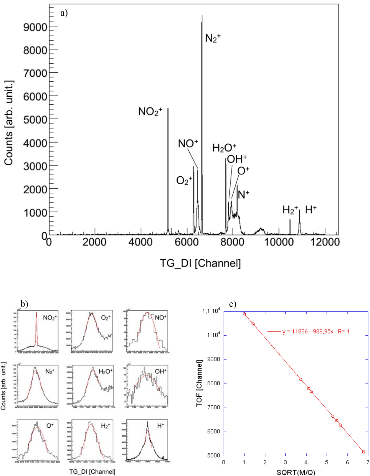
Figure III- 5 a) TG_DI spectrum of NO 2 experiment, b) selected peaks of recoil ions with a Gaussian fitting (red line), c) calibration equation using elected peaks
