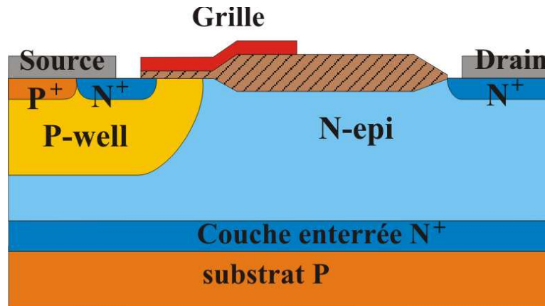
Figure I-24 : Transistor LDMOS LOCOS
