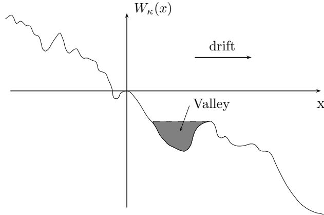
Figure 2.3: A “valley”.
