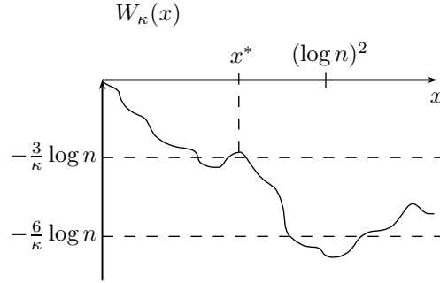
Figure 5.2: \tilde{K}_1
