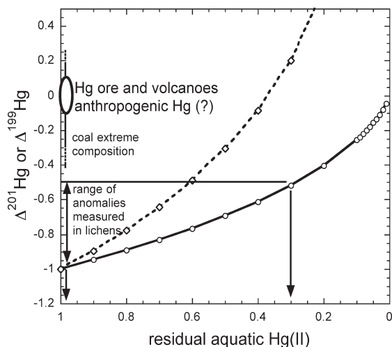
FIGURE 3. The evolution of isotopic anomalies \Delta^{199}\text{Hg} or \Delta^{201}\text{Hg} of \text{Hg}^0 produced by photoreduction of \text{Hg}(\text{II}) as a function of residual \text{Hg}(\text{II}) in solution (dash line, instantaneous composition of \text{Hg}^0 ; full line, cumulative composition of \text{Hg}^0 ). The fractionation of 1‰ between \text{Hg}(\text{II}) and \text{Hg}^0 was calculated from experimental data reported by Bergquist and Blum (14). Note, however, that this value must be taken with precaution for natural environments. Assuming the composition of lichens reflects that of cumulative atmospheric Hg deposition, the measured compositions in lichens from remote areas would suggest that photoreduction is the dominant process for atmospheric Hg emissions. Arrows pointing the x-axis define the percentage (~70%) of aquatic photoreduced \text{Hg}(\text{II}) if the corresponding variation of D^{199-201}\text{Hg} from -1 to -0.5‰ measured in lichens resulted from a reservoir effect. Smaller anomalies most likely reflect the contribution of MDF atmospheric Hg from both natural and anthropogenic sources. Coal composition from ref 29.
