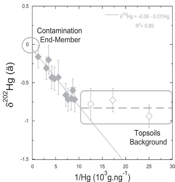
Figure 2. \delta^{202}\text{Hg} (‰) of top soils sampled in the urban area of Metz (Northeastern France) in function of 1/\text{Hg} concentration ( 1000^* \text{g} \cdot \text{ng}^{-1} ). The linear relationship observed for samples with >100 \text{ ng} \cdot \text{g}^{-1} Hg (filled diamonds) indicated a mixing between a contamination source with an end-member of \approx -0.05 ‰ ( \delta^{202}\text{Hg} ) and geogenic Hg (open diamonds). The isotopic composition of the background soil was measured in three soils having low Hg content ( 40 to 80 \text{ ng} \cdot \text{g}^{-1} empty black diamonds) and displayed a \delta^{202}\text{Hg} of -0.82 \pm 0.22 ‰ (2SD, n = 3 ).
