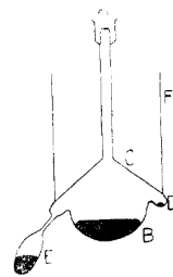
Fig. 2. Cross-section of evaporator for the separation of isotopes (less efficient form).
