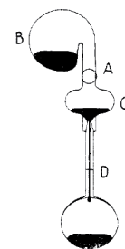
Fig. 3.—Pycnometer.
