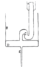
Fig. 4.—Section of efficient evaporator for the separation of isotopes.
