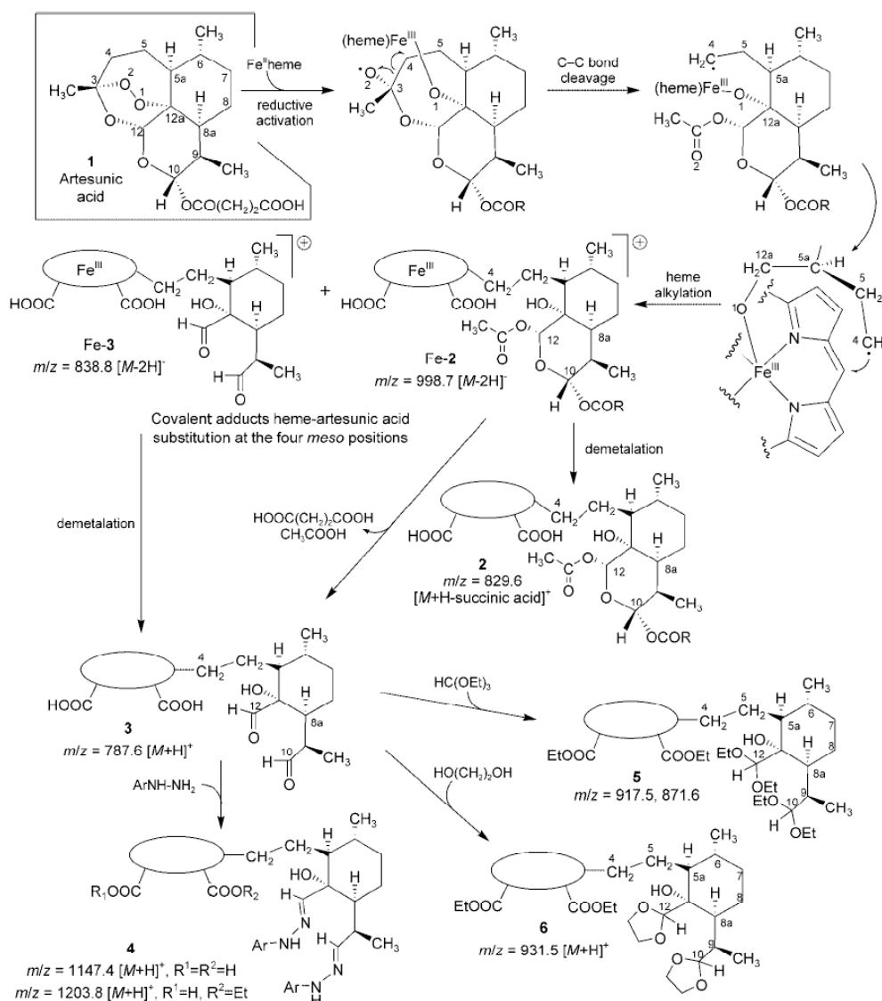
Scheme 1. Alkylation of heme by artesunic acid. Alkylation occurred at four meso positions, only alkylation at the \beta position is depicted. The oval stands for the protoporphyrin-IX macrocycle, R = -(CH_2)_2-COOH , and Ar = 2,4-NO_2-C_6H_3 .
