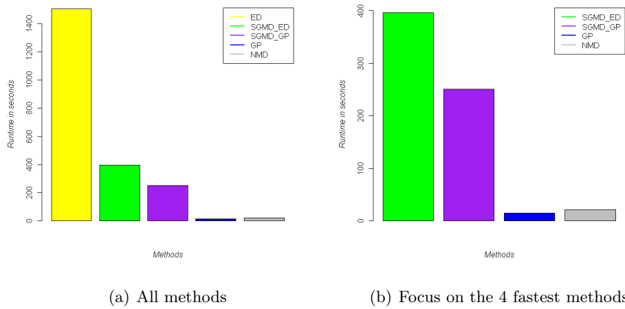
Figure 6.12: Time complexity
