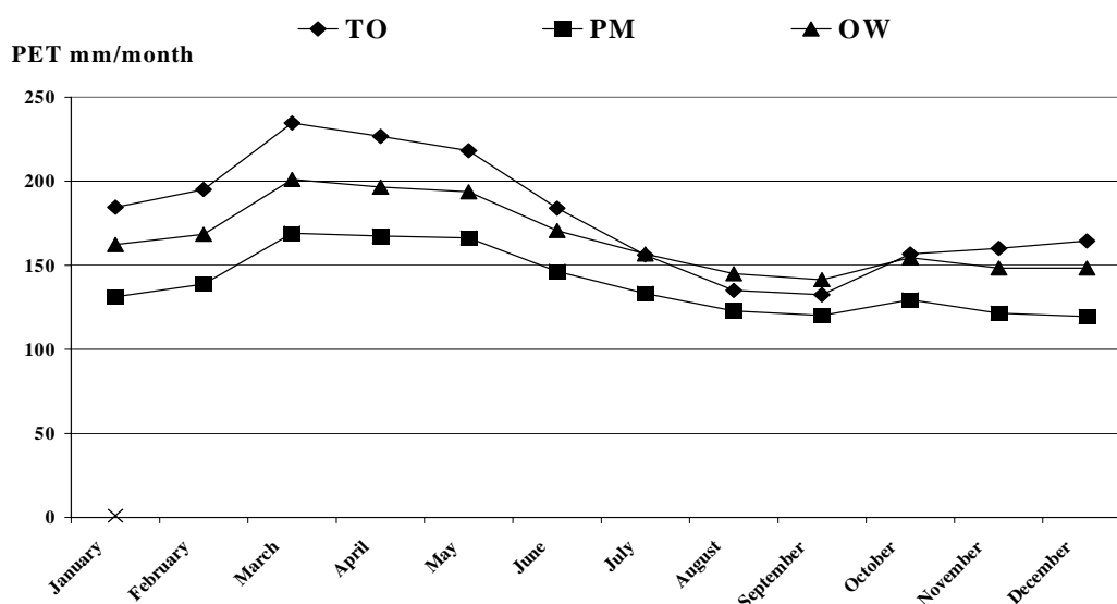
Fig. 3 Comparison of monthly averages of the Thom and Oliver (TO), Penman-Monteith (PM) and Open Water (OW) PET over the period 1950–1995.
