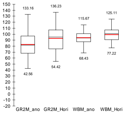
Box plots
