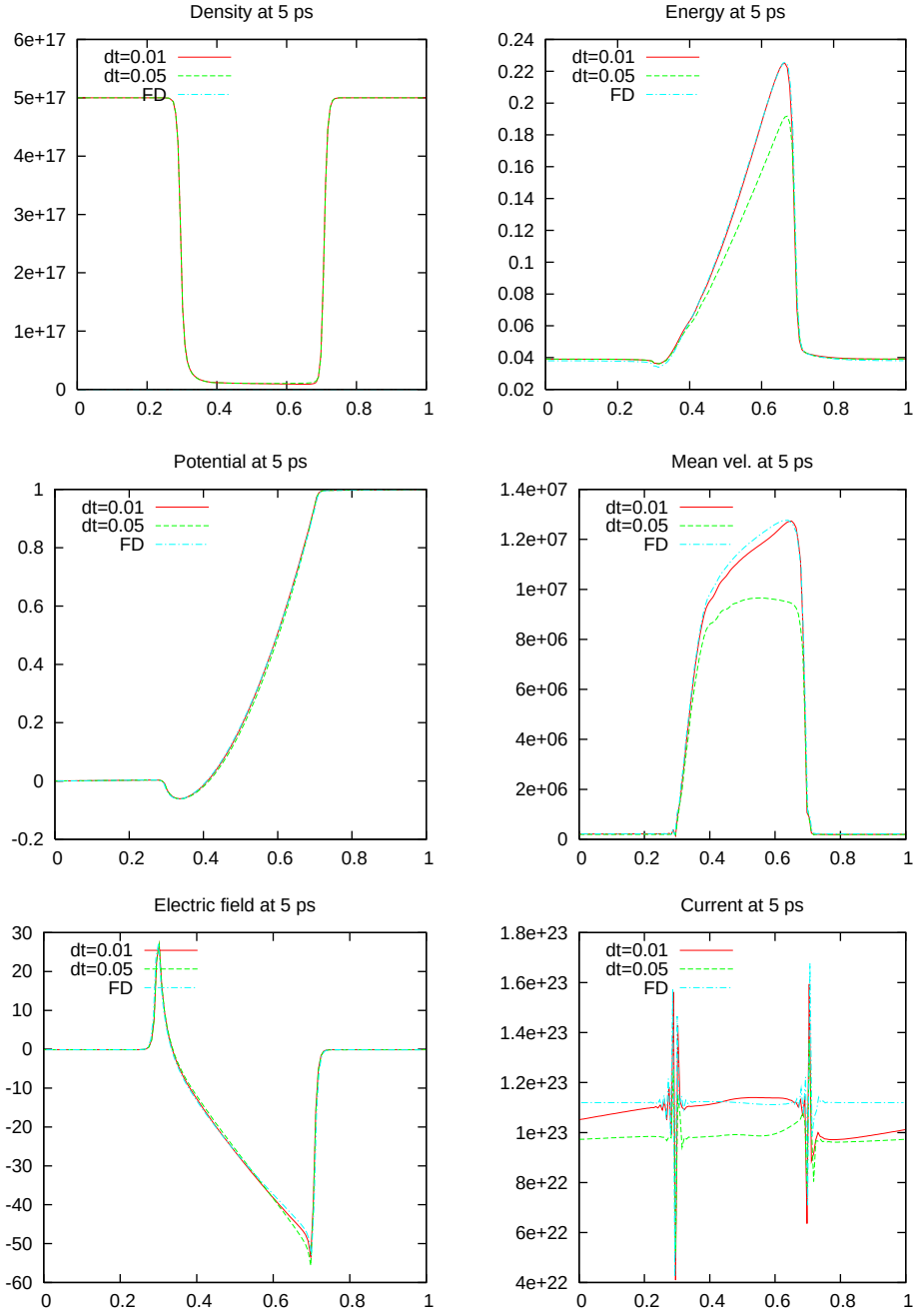
Figure 4: Comparison between some macroscopic quantities of the 400 nm diode at equilibrium (5 ps) given by different time steppings. Top left: density in cm^{-3} ; top right: energy in eV; center left: potential in V; center right: mean velocity in cm s^{-1} ; bottom left: electric field in 10^3 V m^{-1} ; bottom right: current in cm^{-2} s^{-1} . Grids are set 150 \times 40 \times 16 for (x, \omega, \mu) for the W5FD method, 150 \times 71 \times 71 for (x, k_1, k_{23} = \|(k_2, k_3)\|) , \bar{N} = 11 , linear interpolation for collisions, 2nd order TS, for the PW5TS method.
