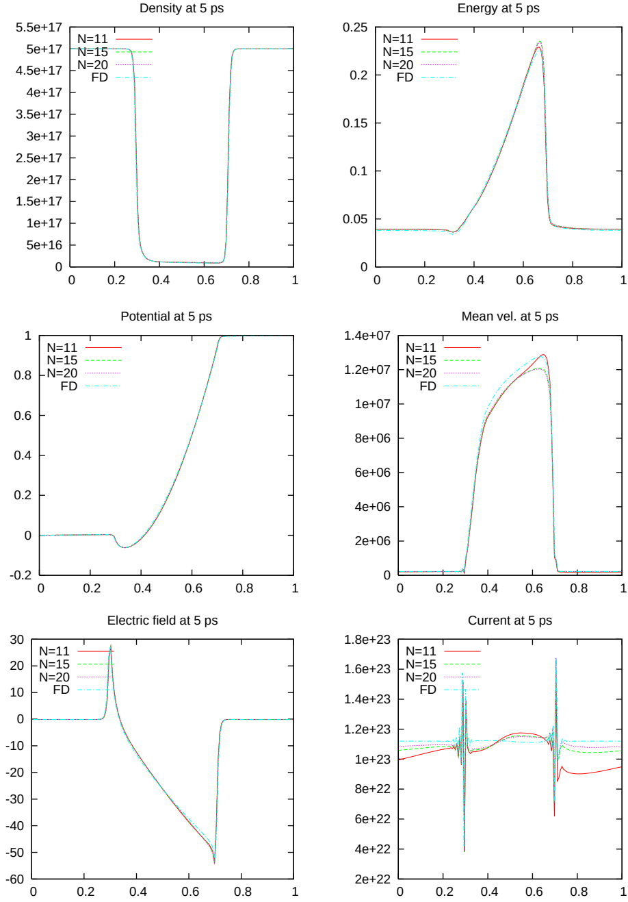
Figure 5: Comparison between some macroscopic quantities of the 400 nm diode at equilibrium (5 ps) given by different \bar{N} . Top left: density in cm^{-3} ; top right: energy in eV; center left: potential in V; center right: mean velocity in cm s^{-1} ; bottom left: electric field in 10^3 V m^{-1} ; bottom right: current in cm^{-2} s^{-1} . Grids are set 150 \times 40 \times 16 for (x, \omega, \mu) for the W5FD method, 150 \times 64 \times 64 for (x, k_1, k_{23} = \|(k_2, k_3)\|) (when \bar{N} = 10 ), \Delta t = 0.01 ps, linear interpolation for collisions, 2nd order TS, for the PW5TS method.
