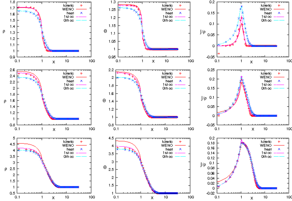
Figure 12: Su-Olson test: Left column: comparison of densities \rho ; middle column: comparison of temperatures \Theta ; right column : comparison of reduced fluxes \varepsilon J/\rho in log-log scales for the solutions after time 1, 3 and 10 time units respectively (from top to bottom) computed with the kinetic, the heat equation, the first and the zeroth order closure methods for \varepsilon = 1 . The initial data is f_0 = \rho_0 = \Theta_0 = 1 .
