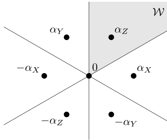
Figure 3.2: The six Weyl chambers of \mathrm{SL}(3, \mathbb{C}) . The fundamental chamber \mathcal{W} is shaded.
