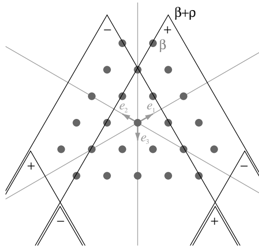
Figure 6.3: The six cones appearing in the partial derivative of the Kostant multiplicity formula, and their associated signs.
