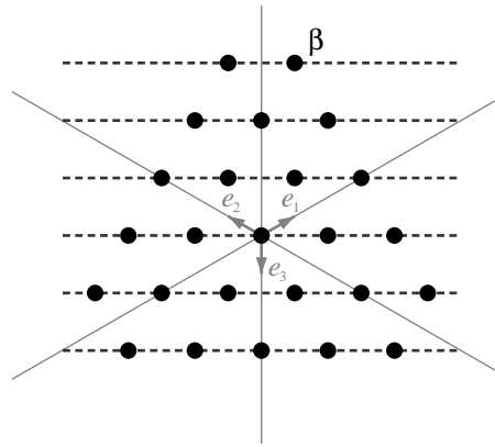
Figure 6.2: Decomposition of the representation \Gamma^\beta into \mathfrak{s}_X -strings.
