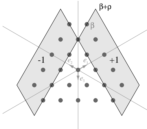
Figure 6.4: Support of the signed characteristic functions.
