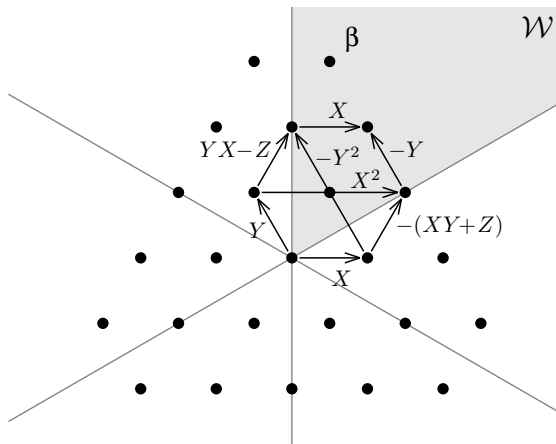
Figure 6.1: Pictorial description of the BGG-complex in the K -type with highest weight \beta = 2\alpha_X + 3\alpha_Y . Dots represent weight spaces, and arrows map between them.
