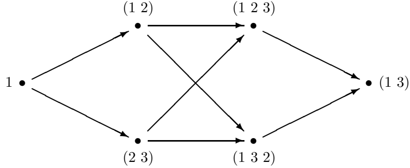
Figure 3.3: Directed graph structure for the Weyl group of SL(3, \mathbb{C}) .
