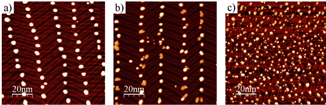
FIGURE 3.8 – Images STM 100 \times 100 \text{ nm}^2 (a) Co pur , \theta = 0,05 \text{ MC} (b) Co 54 Pt 46 , \theta = 0,05 \text{ MC} (c) Co 25 Pt 75 , \theta = 0,01 \text{ MC}
