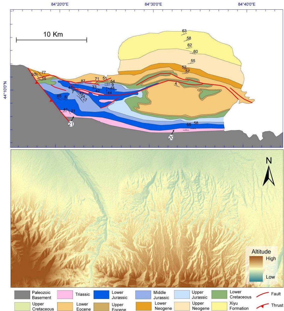
Figure 4-21. Geological map (b) DEM of the Tuositai anticline in the Wusu area.
