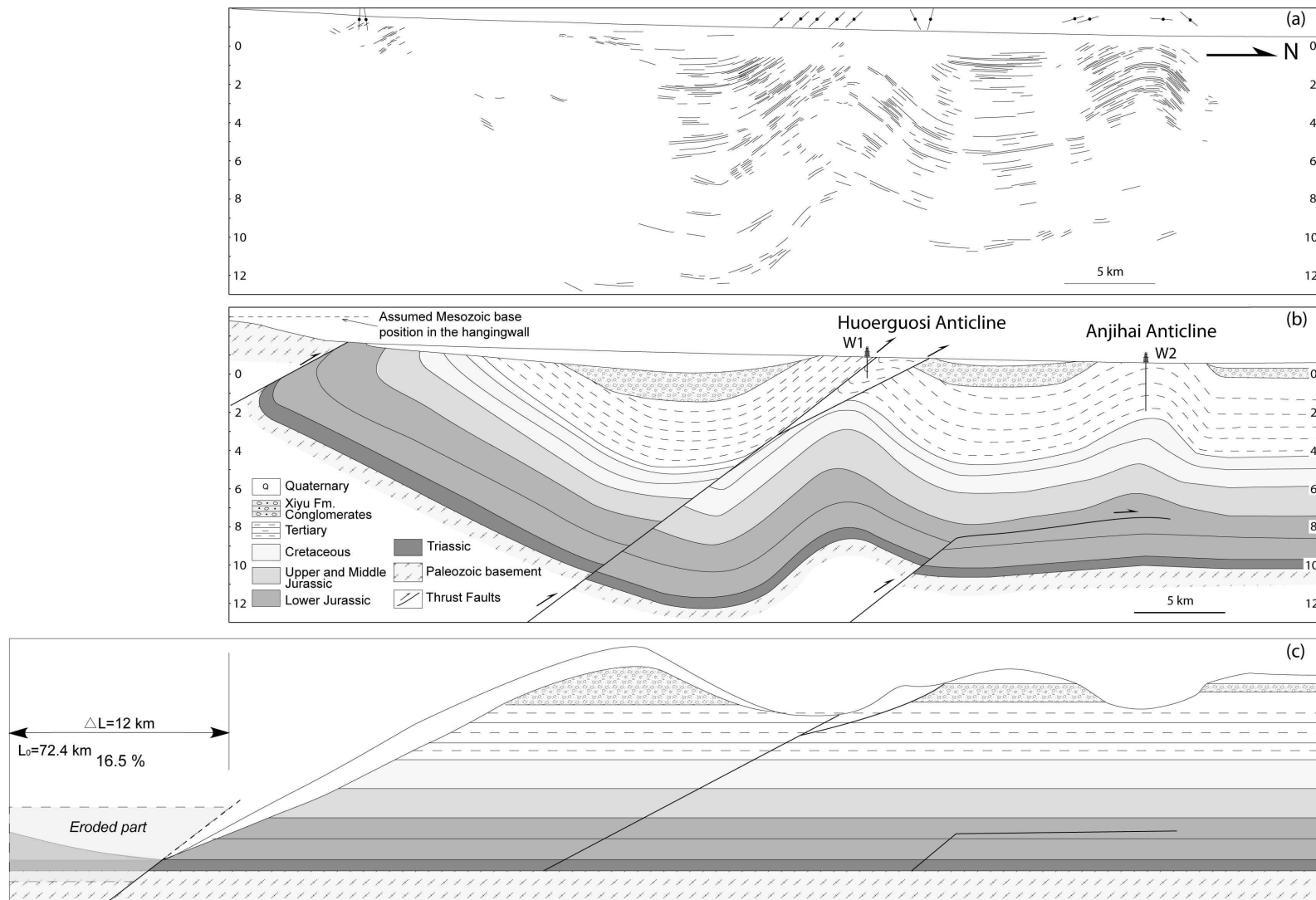
Figure 5-7. (a) Linedrawing of the seismic profile along the Jingou He section associated with formation limits and dip angles on the field. (b) Interpretation of the seismic profile. (c) the restored section along Jingou He.
