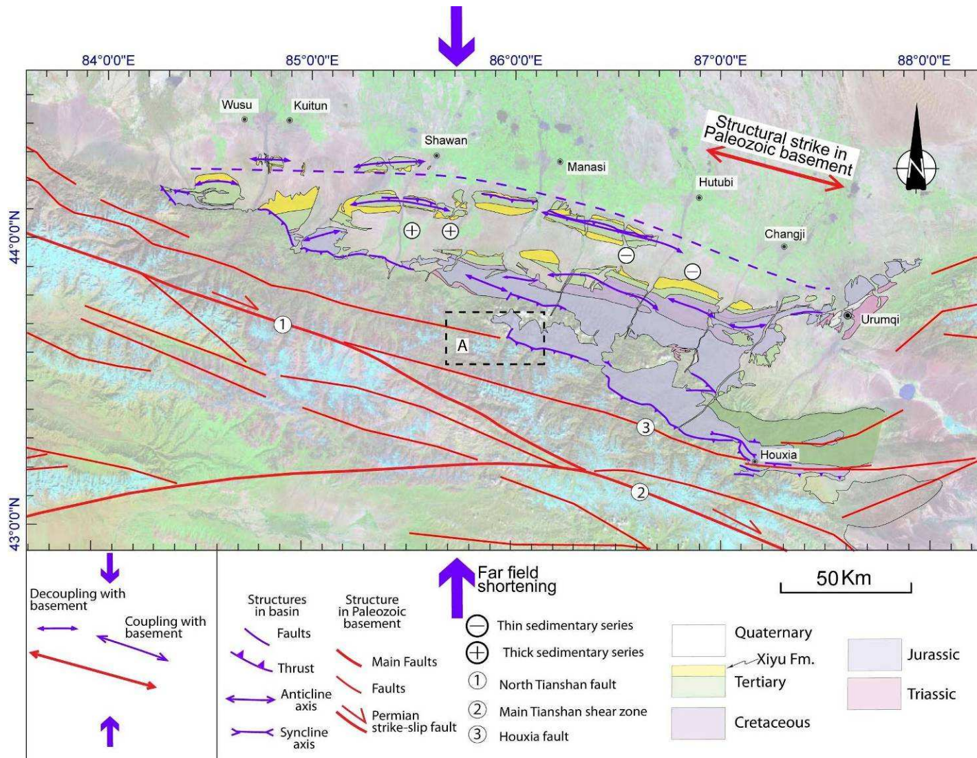
Figure 6-8. Geological map of the northern piedmont of Tian Shan, with comparison of the location and orientation of the Paleozoic and Cenozoic structures.
