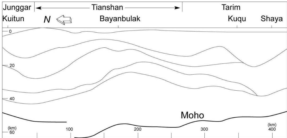
Figure A-15. Schematic crustal structure along the Kuitun-Shaya profile in the Tian Shan area. The overstriking line indicates the Moho (after Lu et al., 2000).
