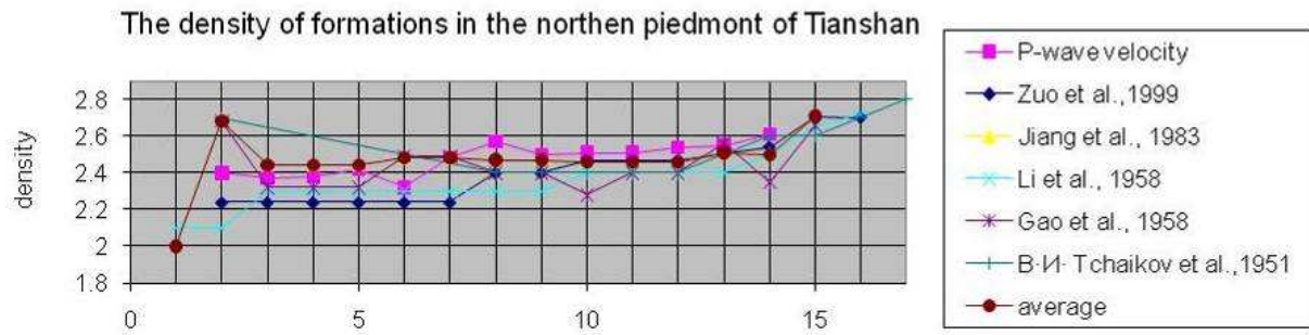
Figure A-12. Density distribution from different resoures. 1 to 15 indicate Quaternary (1), Xiyu Fm. (2), Dushanzi Fm. (3) , Taxi He Fm. (4), Shawan Fm. (5), Anjihai Fm. (6), Ziniquanzi Fm. (7), Dongou Fm. (8), Tugulu Fm. (9), Upper Jurassic (10), Middle Jurassic (11), Lower Jurassic (12), Triassic (13), Permian (14), Carboniferous (15), Devonian (16) and crystal basement.
