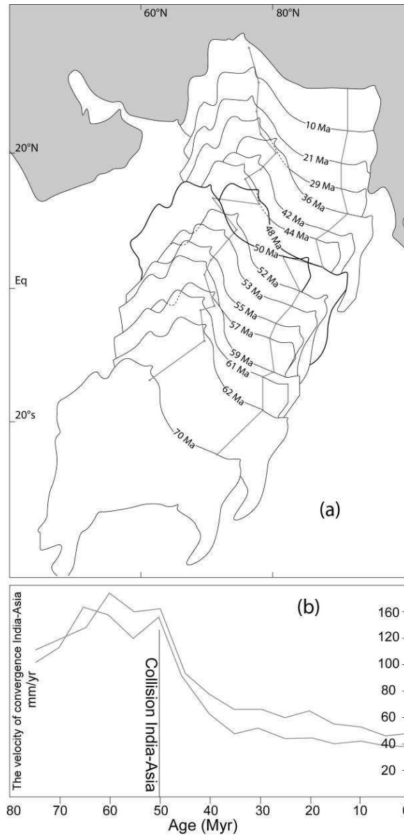
Figure 2-2. (a) Cenozoic northward drift of India, relative motion of India with respect to Eurasia, kept arbitrarily fixed in its present position. The two traces indicate two points located on the Indian continent near the northern margin. Black-bold outlines indicate the initiation of India-Asia collision. (b) The velocity of the two points above move toward the Asia plate. India-Asia collision time was suggested by the sudden decrease (~ 50 Ma) (Patriat and Achache, 1984; Avouac and DeWver, 2002).
