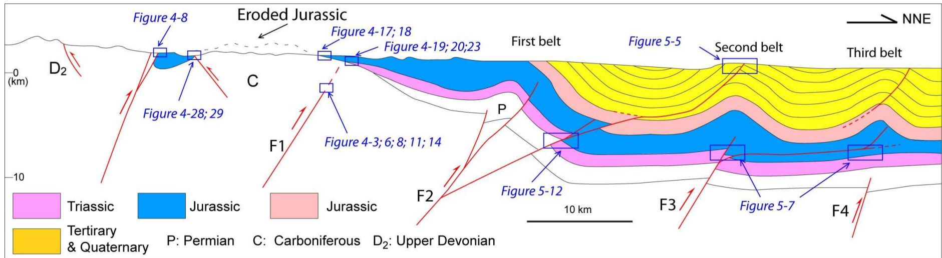
Figure 6-5. Sketch diagram of the structure and developing model for the northern Tianshan. Numbers indicate the faults in the basement (modify after Qi et al., 2007).
