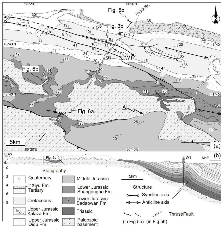
Figure 3-5. (a) Simplified geological map of the Hutubi He area. 'A' indicates the unconformity between Middle Jurassic and Carboniferous basement. There, Triassic and Lower Jurassic are apparently lacking. (b) Geological cross-section of along the Hutubi He constrained by field data, seismic profile and drill well W1.
