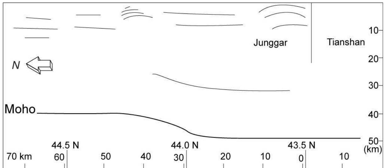
Figure A-16. Sketch of the crustal structure in the northeastern Tian Shan margin along Manasi He (after Wang et al., 2004).
