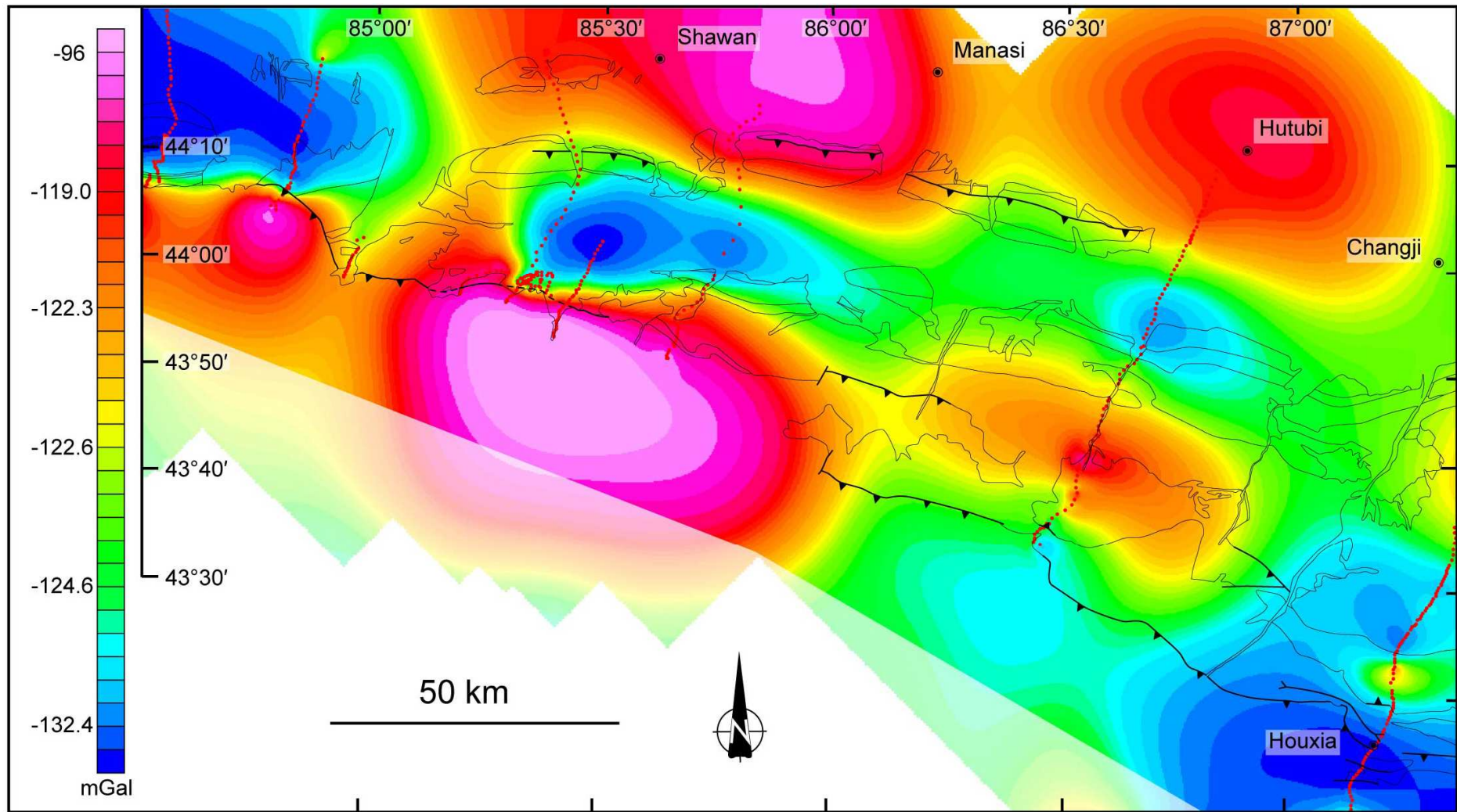
Figure 5-18. Bouguer anomaly map in the northern piedmont of Tian Shan with locations of gravity stations (red dots). Major geological limits are drawn. See Figure 4-1 for details of geological boundaries.
