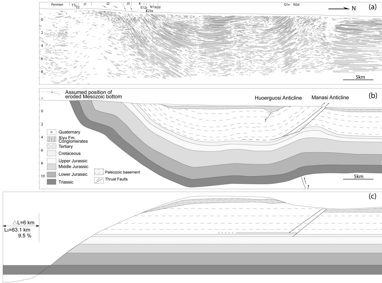
Figure 5-9. (a) Linedrawing of the seismic profile along the Qingshui He section associated with geological formation limits and dip angles measured on the surface. (b) Interpretation of seismic profile. (c) Restored section along the Qingshui He.
