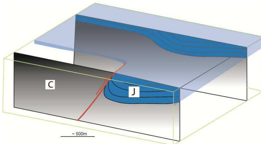
Figure 4-35. Sketch diagram shows the lateral structural variation. This example can be seen in the southern Hutubi (Figure 4-1, N^{\circ} 23 ).
