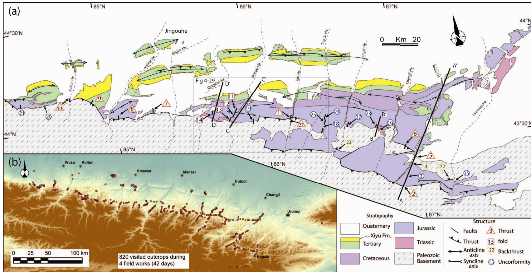
Figure 4-1. Geological map of the northern piedmont of Tian Shan with locations of field observations along the front. The upper map (a) shows the observed locations of cross-sections and outcrops (modified after He et al., 2005). Red triangles with numbers: thrust contact outcrops, purple squares: fold-type contact outcrops, orange reversed triangle: backthrusts in the mountain and blue circles: unconformity contact between range basement and basin sediments. All the numbers will be found in the pictures displayed and presented in this chapter. Lower framed map (b) is the DEM of the northern piedmont of Tian Shan with red circles points indicating 820 visited outcrops during 3 field trips.
