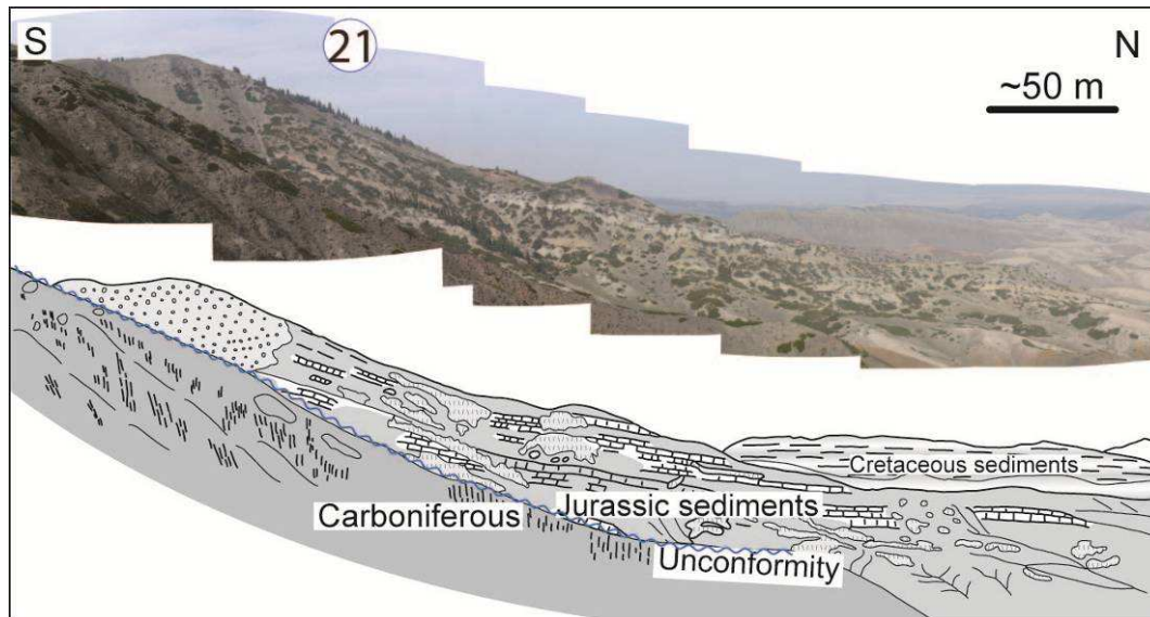
Figure 4-23. Jurassic series overlies on the Paleozoic basement with a monocline towards north at the southern end of Wusu area.
