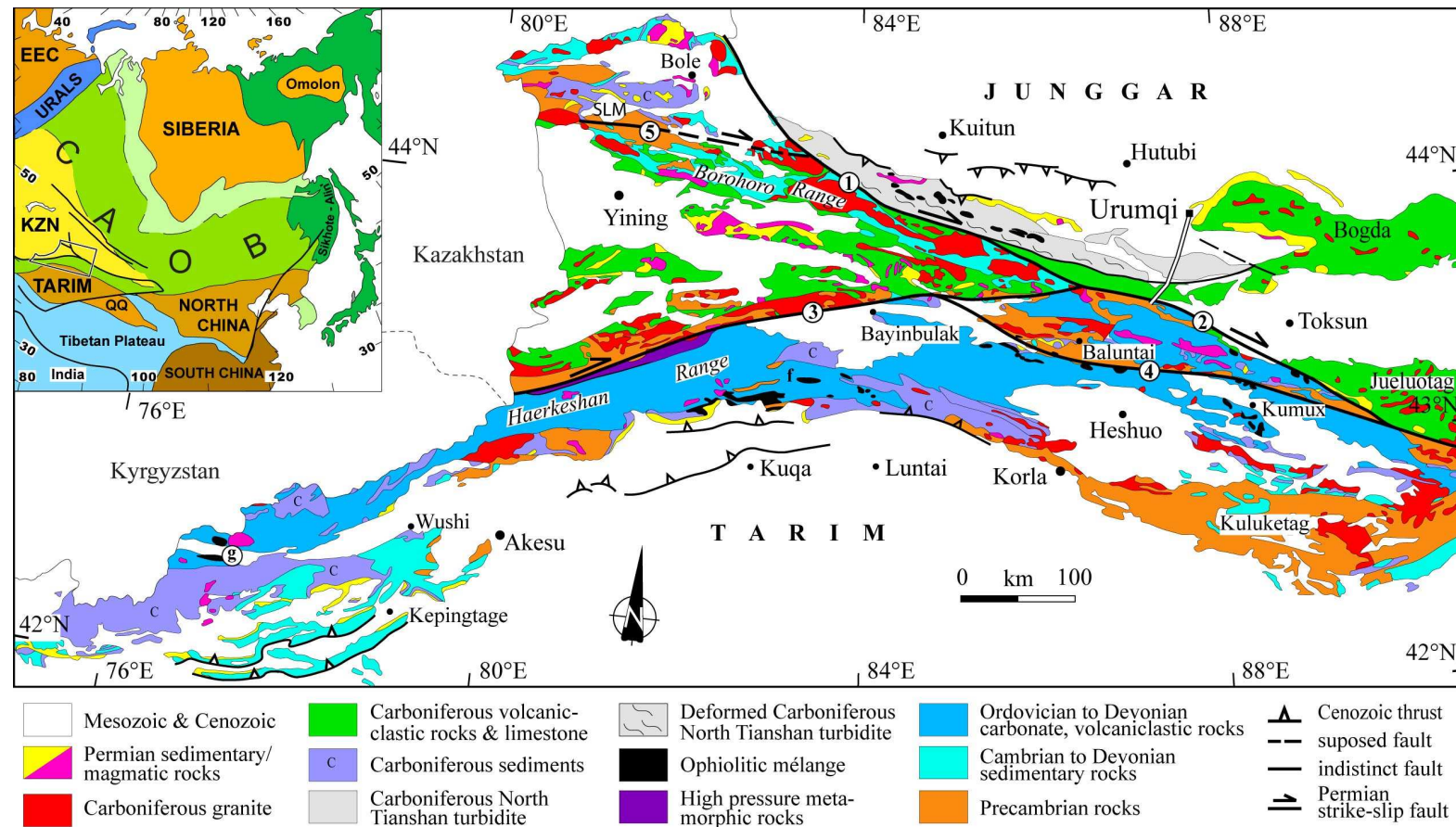
Figure 2-4. Geological map of the Chinese western Tian Shan belt (after Wang et al., 2008). Numbers in circle refer to the main faults: 1, North Tian Shan fault (NTF); 2, Main Tian Shan shear zone (MTSZ); 3, Qingbulak-Nalati fault (QNF); 4, Sangshuyuanzi fault; 5, Jinghe fault. Inset shows location of the Tian Shan Belt in Central Asia (modified from Jahn, 2004). Abbreviations: CAOB, Central Asian Orogenic Belt; EEC, Eastern European Craton; KZN, Kazakhstan; QQ, Qaidam-Qinling.
