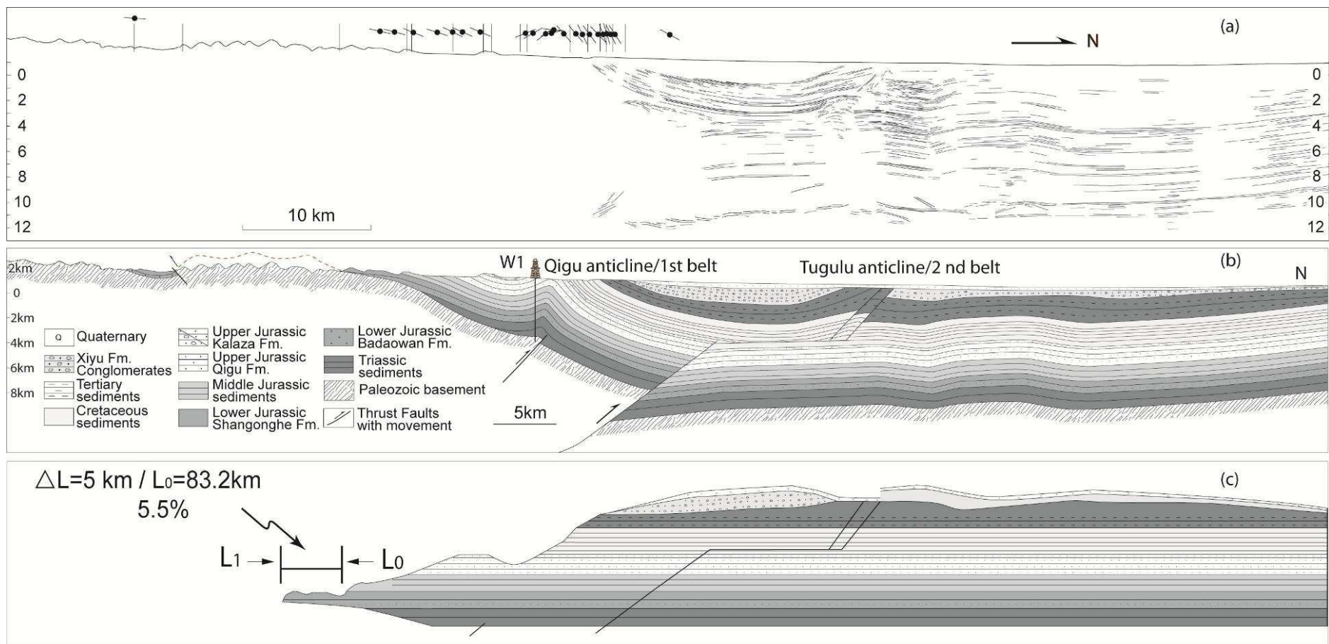
Figure 5-12. (a) Linedrawing of the seismic profile along Hutubi He section (b) Interpretation of seismic profile. (c) Restored section along the Hutubi He, taking the Jurassic layers as marker.
