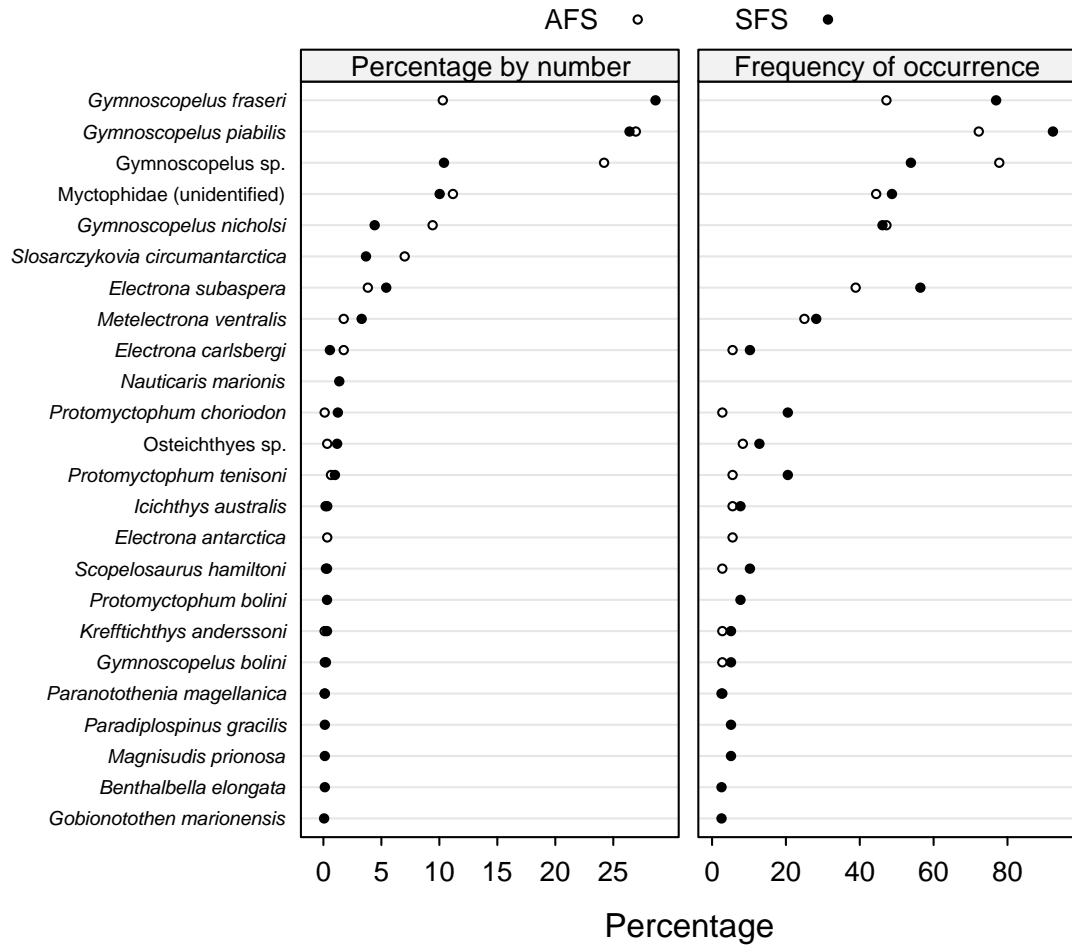
Figure 2.6. Percentage by number (of total prey items) and relative frequency of occurrence of identified prey in scat samples of Antarctic (AFS) and subantarctic (SFS) fur seals from MAE, Iles Crozet. Only those species with relative frequency or frequency of occurrence higher than 1% are shown
