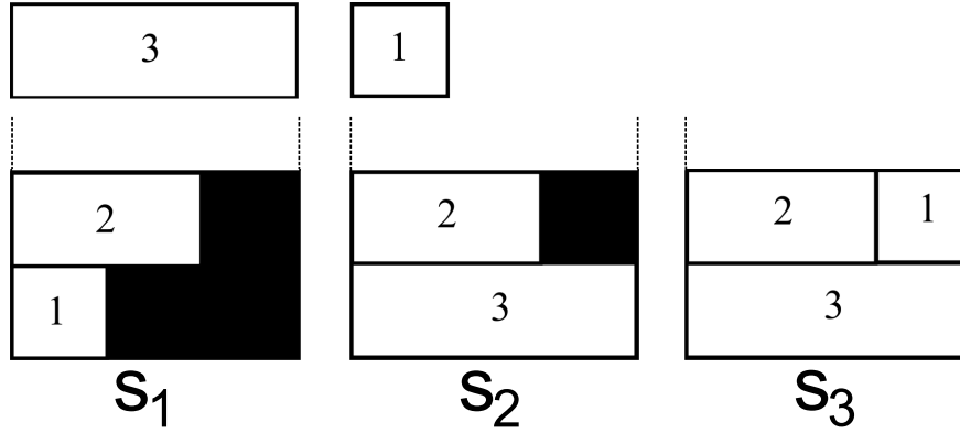
FIGURE 4.1 – Soient r_1 le carré unitaire (i.e. w_1^r = h_1^r = 1 ) et k = 2 . f(s_1) = 9 car E \neq \emptyset , M_w = w_3^r = 3 , M_h = h_3^r = 1 , \alpha = 1 , \delta = (3.1)(2.0) + (3.2)(2.0) = 6 , et M_a = 2 . De même, f(s_2) = 1 car E \neq \emptyset , M_w = 1 , M_h = 1 , \alpha = 1 , \delta = 1 , et M_a = 1 . f(s_3) = 0 car E = \emptyset et \alpha = 0 .
