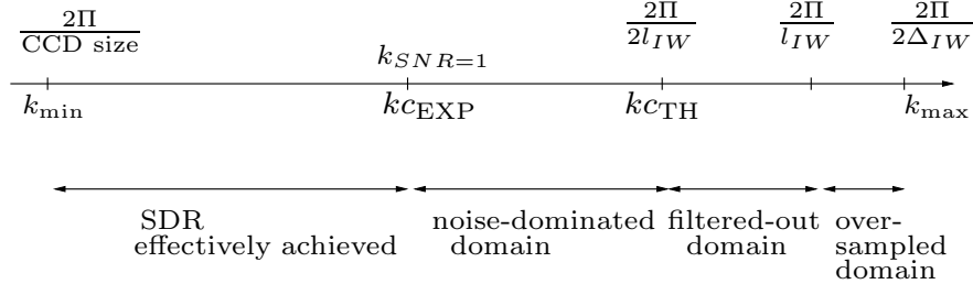
Figure 2.3: Different wavenumber regions of a typical PIV spectrum of turbulent flow
