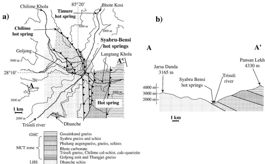
Fig. 2. a) Geological map of the Syabru-Bensi area simplified from Macfarlane et al. (1992) showing the location of studied hot springs and cross section AA'. Topographic contours are taken from the 1:50 000 sheet number 2885 14 (Survey Department of Nepal, revised 1996). b) N40°E geological section of the MCT zone along AA'.
