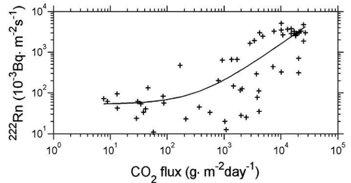
Fig. 8. Radon-222 versus carbon dioxide flux. The \text{CO}_2 flux at each radon-222 measurement point is interpolated from the map (Fig. 3) when not available at the same location. The line corresponds to a robust least square fit. The radon flux of this line is given as 77.7 + 0.156 \times \text{CO}_2 flux.
