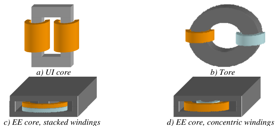
Figure III.2: Two-cell ICTs using different core shapes.
