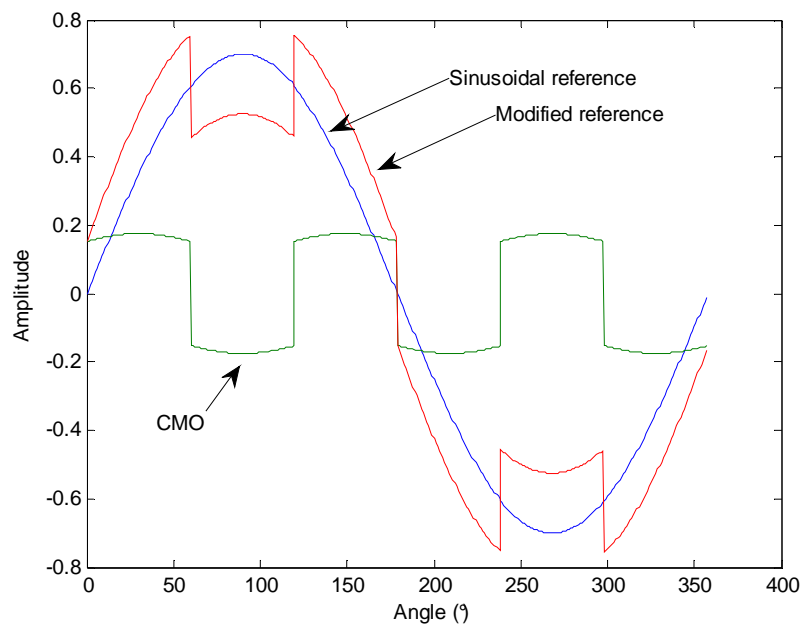
Figure V.36: Modulation waveforms of PWMBC method ( M_i=0.7 ).
