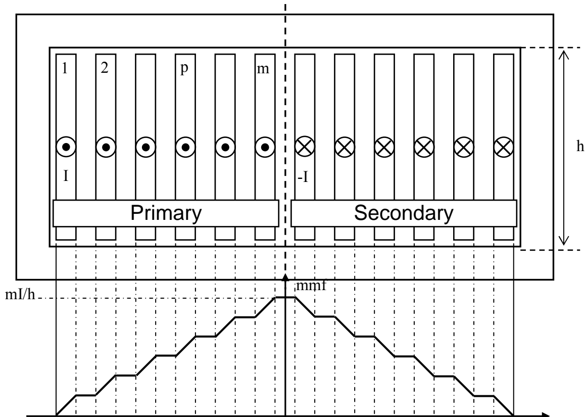
Figure II.8: Transformer parameters used to explain Dowell's formula.
