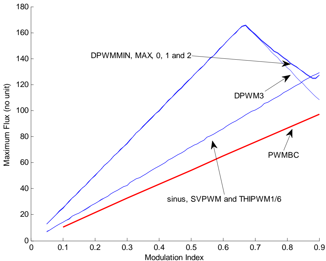
Figure V.40: Maximum flux ripple for different PWM methods.
