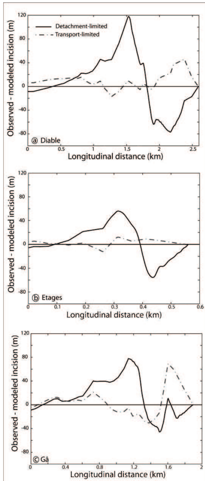
Figure IV.3.12. Difference between observed and modeled incision as a function of longitudinal distance for the transport- (dashed line) and detachment-limited (continuous line) models for (a) Diable, (b) Etages and (c) Gâ streams.
