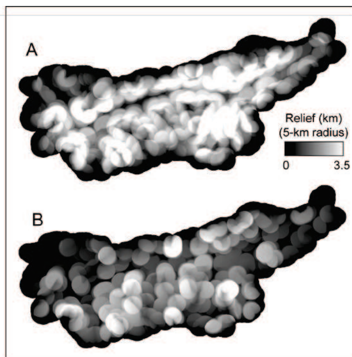
Figure III.4.9. Rhône basin relief (ridge line to valley bottom relief) calculated using a 5-km radius for both present-day (A, R_{max} = 3.5 km and R_{mean} = \sim 1.8 \pm 0.6 km) and pre-glacial (B, R_{max} = 2.5 km and R_{mean} = \sim 1.6 \pm 0.5 km) topographies.
