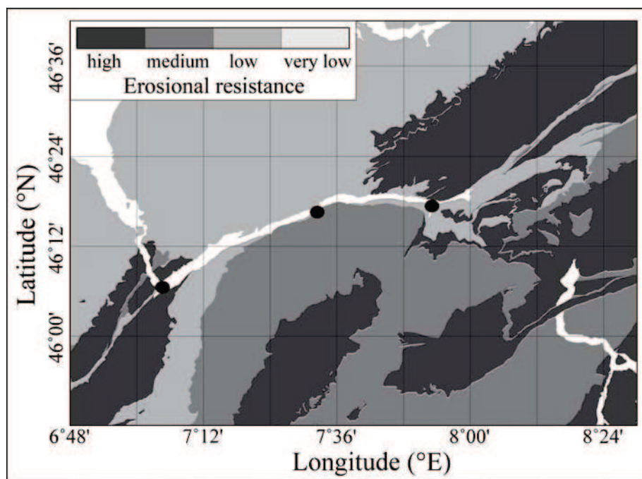
Figure IV.2.15. Simplified spatial distribution of lithologies in the Valais area, illustrating the spatial variability in erosional resistance [ Kühni and Pfiffner, 2001b; Schlunegger and Hinderer, 2001; Norton et al., 2010a ].
