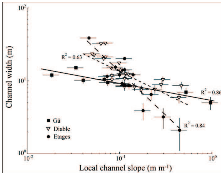
Figure IV.3.7. Channel width and slope variations (logarithmic plot) for the Etages (circles and dashed curve), Diable (inverted triangles and dot curve) and Gâ (squares and solid curve) streams. Note that the exponent of the power-law correlation between local gradient and channel width (Etages: -1.23 \pm 0.36 ; Diable: -0.59 \pm 0.21 ; Gâ: -0.23 \pm 0.09 ) appears to be modulated by tributary drainage area (Etages: 14 km 2 ; Diable: 20 km 2 ; Gâ: 42 km 2 ). Errors on slope ( \pm 20\% ) and width ( \pm 1 m) values are indicated.
