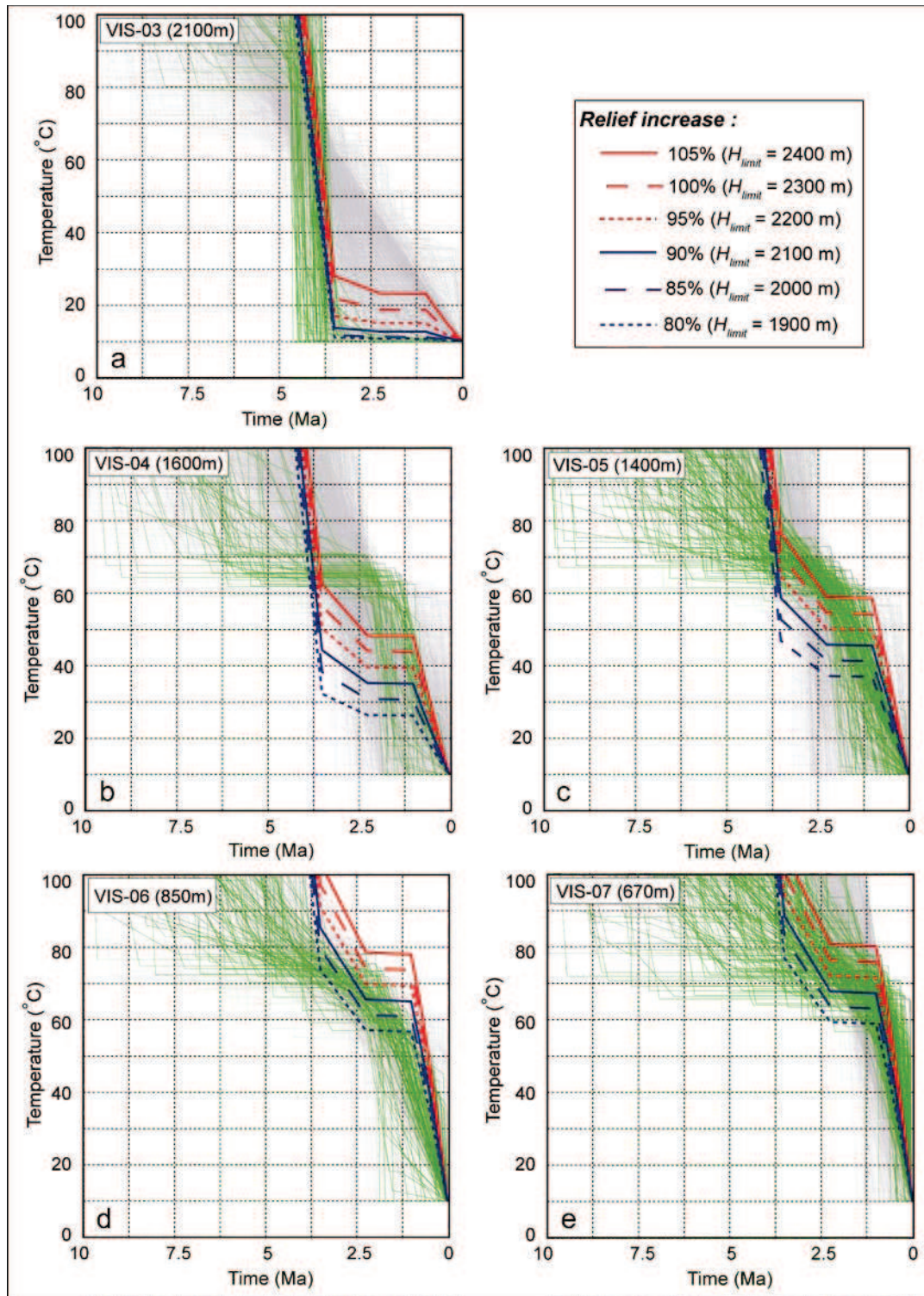
Figure III.3.7. Cooling paths for VIS samples inferred from ^4\text{He}^3\text{He} and Pecube models (see Figures III.3.1 and III.3.2 for sample locations). Green/grey lines show respectively good and acceptable ^4\text{He}^3\text{He} modeled cooling paths for VIS-03 (a), -04 (b), -05 (c), -06 (d) and -07 (e) [Valla et al., submitted, a]. Thick coloured lines (blue and red) show modeled cooling paths simulating relief development carving of various amplitudes (80 to 105% relief increase, see legend for colours code) since \sim 1 Ma. See text for other parameters.
