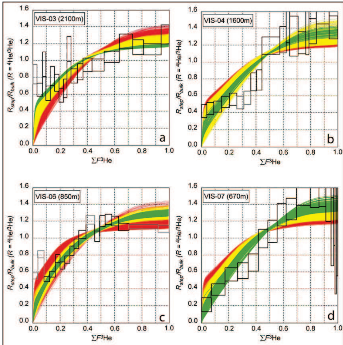
Figure III.2.5. Observed {}^4\text{He}/{}^3\text{He} ratios of VIS-03 (a), -04 (b), -06 (c) -07 (d). The measured {}^4\text{He}/{}^3\text{He} ratios of each released step ( R_{step} ) are normalised to the bulk ratio ( R_{bulk} ) and plotted versus the cumulative {}^3\text{He} release fraction \Sigma F^3\text{He} . Open black boxes indicate 1 standard error (vertical) and integration steps (horizontal); open grey boxes show released steps that were excluded from the misfit calculation (see section III.2.6 for discussion). Colored lines show the predicted {}^4\text{He}/{}^3\text{He} ratio evolution diagrams. Models shown in red and yellow are excluded by the {}^4\text{He}/{}^3\text{He} data, whereas the green cooling paths are permitted.
