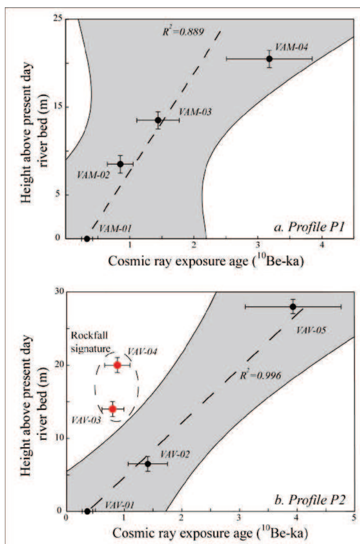
Figure IV.3.17. Vertical profiles P1 (a) and P2 (b) (see Figure IV.3.15 for locations) and calculated CRE ages. Errors on height measurements ( \pm 1 m) and CRE ages (see Table IV.3.2) are given. Best linear fits (dashed line, a: Slope = 11 \pm 2 m ka^{-1} ; R^2 = 0.889 ; b: Slope = 7.5 \pm 1.5 m ka^{-1} ; R^2 = 0.996 ) and 95% confidence interval (grey zone) are also shown.
