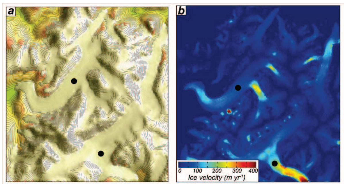
Figure IV.2.10. Late-Glacial (~16-17 ka) ice-extent reconstruction and predicted ice velocities. (a) Ice-extent modeling with an input ELA shift of -800 m [Dorthe-Monachon, 1986; Coutterand and Nicoud, 2005; Norton and Hampel, 2010], showing the progressive glacier retreat within the Arve and Baltée valleys, and (b) predicted horizontal ice velocities (see text for discussion). Dots indicate location of towns of Chamonix and Courmayeur.
