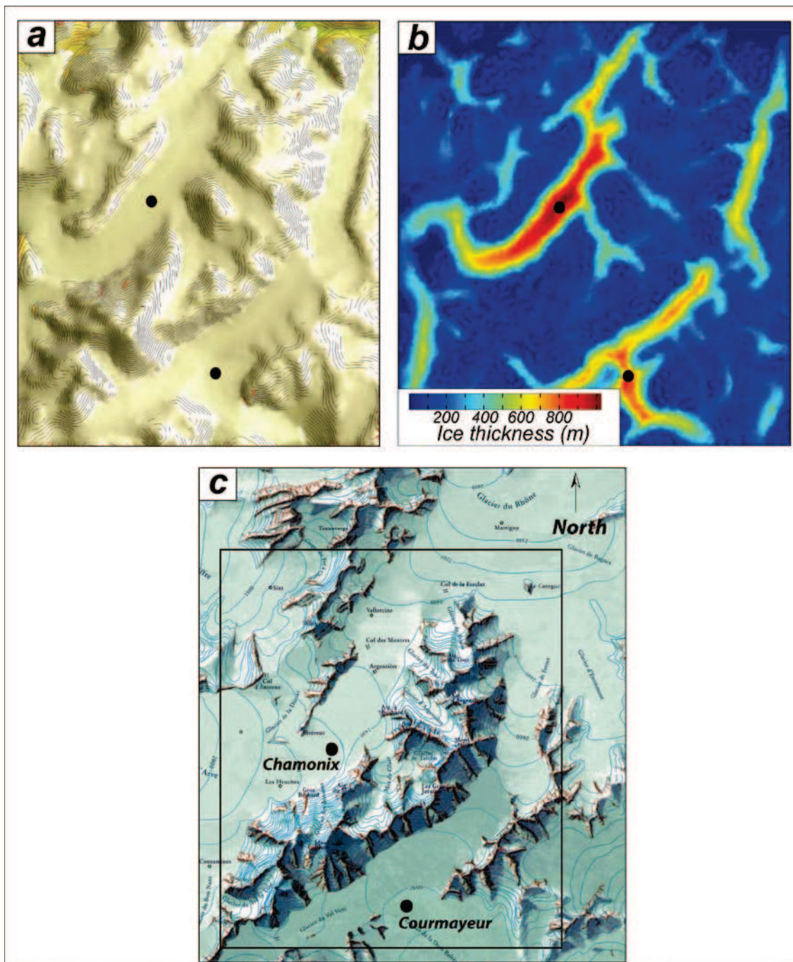
Figure IV.2.9. Last Glacial Maximum (LGM ~20-21 ka) ice reconstructions. (a) Ice-extent simulation using the SPMIce model with an input ELA shift of -1280 m [Ivy-Ochs et al., 2006; van der Beek and Bourbon, 2008; Coutterand, 2010; Norton and Hampel, 2010], (b) associated ice-thickness pattern, and (c) ice-extent reconstruction (box indicates model extent) based on trimline distribution [Coutterand and Buoncristiani, 2006].
