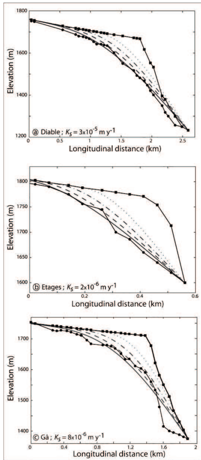
Figure IV.3.11. Initial glacial (squares) and present-day fluvial (circles) profiles for (a) Diabie, (b) Etages and (c) Gâ streams; and profile evolution predicted by the best-fit transport-limited model ( m_s = n_s = 1 ; K_s as indicated in the plots). Thick lines show profiles at 5-ky intervals during the model run (dotted: 5 ky; dashed-dotted: 10 ky; dashed: 15 ky and solid: 20 ky).
