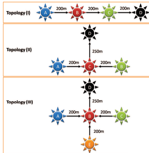
Figure 4.4: Topology (I) is a chain topology, where the source nodes(A,B and C) send data to D. Topology (II) is a T topology, where the source nodes(A,B and C) send data to D. And topology (III) is a tree topology, where the source nodes(A, B, C and E) send data to D.
