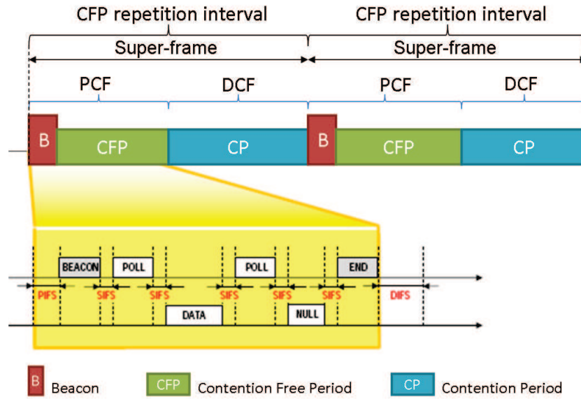
Figure 1.2: PCF access method
