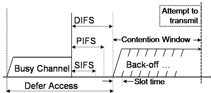
Figure 1.4: The Inter-frames for accessing the channel
