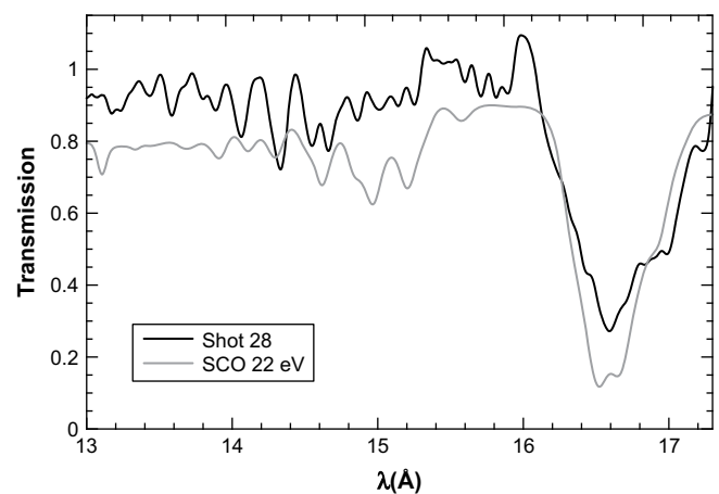
Fig. 7. Experimental transmission of iron (shot 28 on Fig. 4) compared with a SCO calculation performed for a temperature of 22 eV and a density of 4 \text{ mg}/\text{cm}^3 with a convolution corresponding to a 4 eV resolution.
