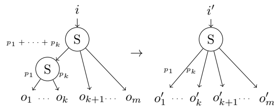
(b) CompactSS
