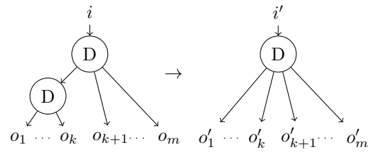
(a) CompactDD
