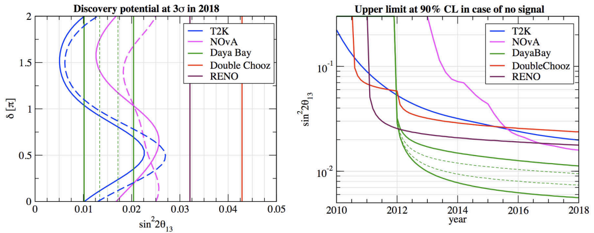
Figure 4.15: Left panel: discovery potential expected in 2018 for the five running/upcoming experiments in the plane \sin^2 2\theta_{13} - \delta . Straight lines are the reactor experiments and curved lines are the accelerator ones. Right panel: evolution of the 90% C.L. sensitivity to \sin^2 2\theta_{13} as a function of time. In both plots, the several Daya Bay curves correspond to different possible systematic uncertainties [103]. The best discovery potential is for the accelerators while the best sensitivity is for the reactor experiments.
