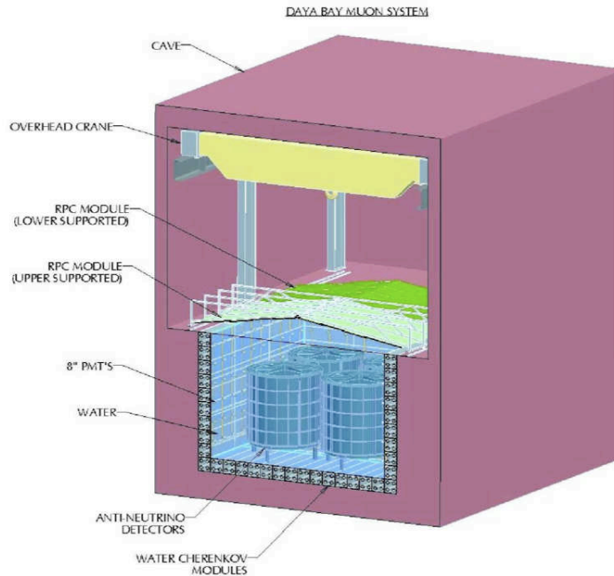
Figure 4.5: The Daya Bay muon veto system and the 4×20t detectors.
