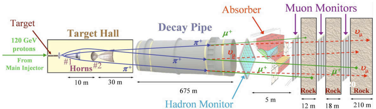
Figure 4.7: Illustration of a neutrino beam principle with the NuMI beam at FermiLab (Chicago, U.S.A) [117].
