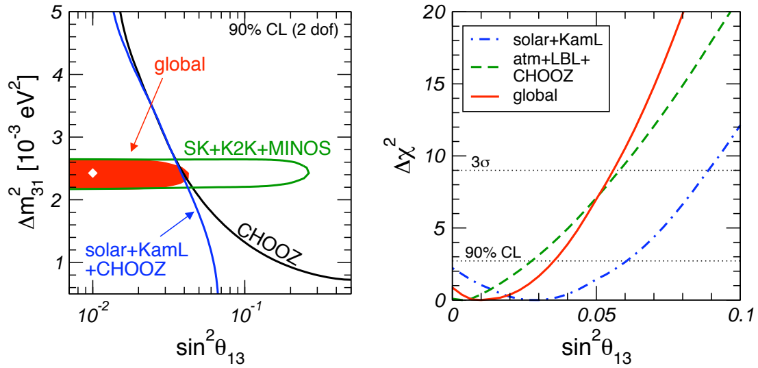
Figure 3.19: Global fit to oscillation experiments data. One can see that the solar sector’s \Delta\chi^2 favors a non-zero value of \theta_{13} reachable by the new generation of oscillation experiments [100]
